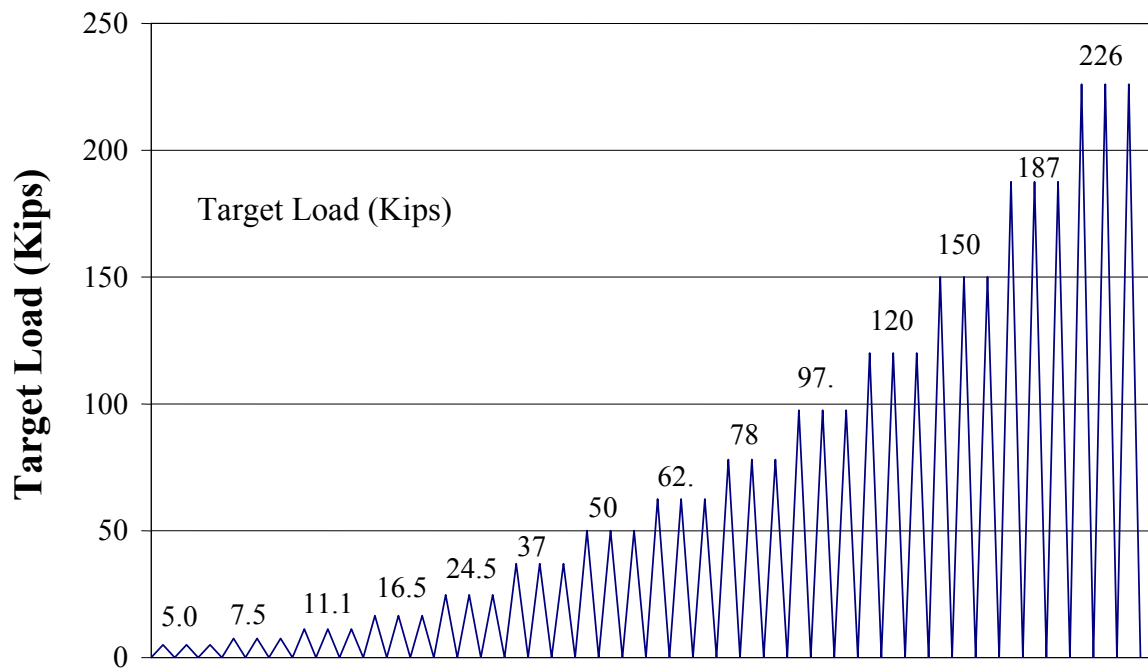
Figure 2.15: March target load increments.
