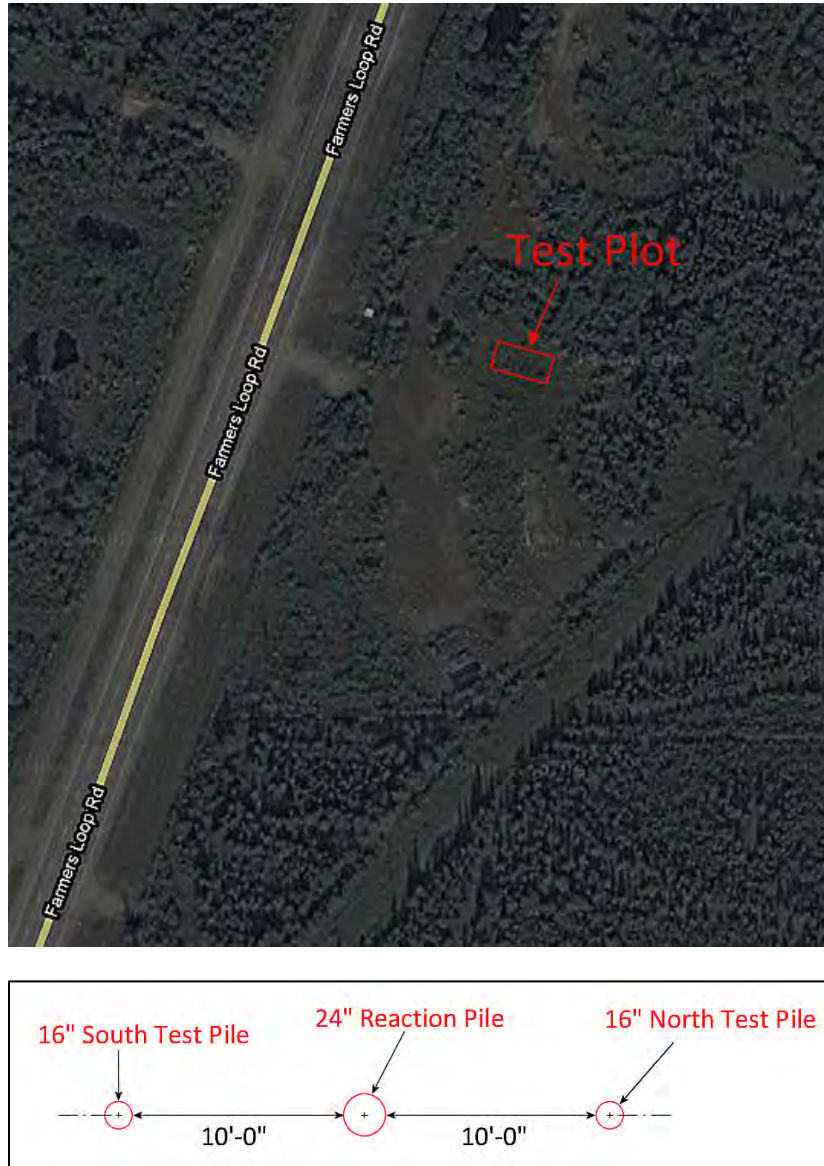
Figure 2.2: Test pile location and layout plan view (Google n.d.).
