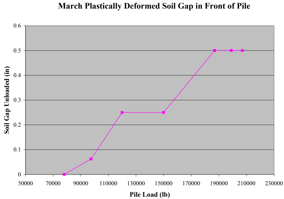
Figure 2.33: Plastically deformed soil gap in front of pile, March test.
