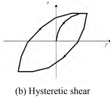
Figure 4.4: von Mises multi-surface kinematic plasticity model (Yang 2000; Yang et al. 2003).
