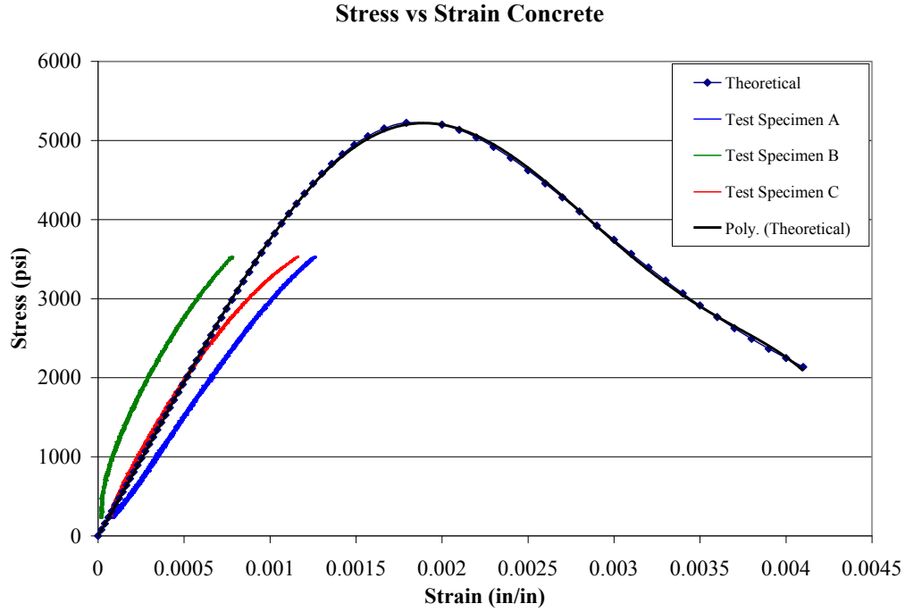
Figure 2.42: Concrete stress-strain behavior, experimental and theoretical.
