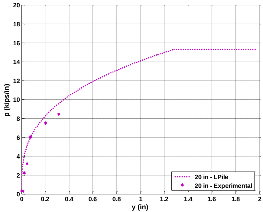
Figure 6.8: Proposed p - y curves vs. back-calculated p - y values at depths of (a) 5 inches, (b) 10 inches, (c) 15 inches, and (d) 20 inches.
