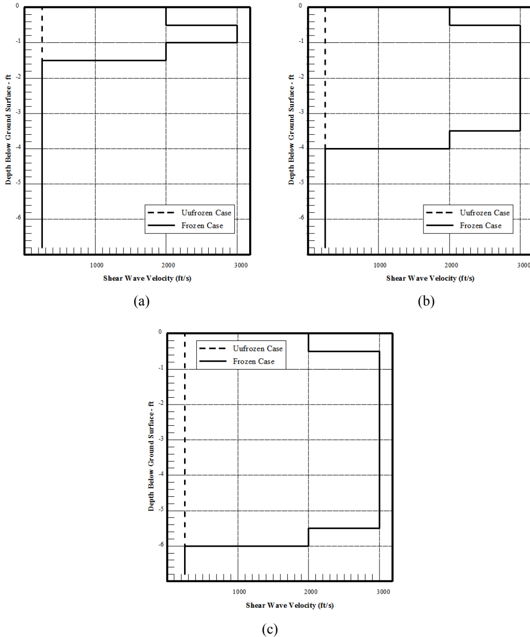
Figure 4.12: Shear wave velocity profile of the test site: (a) frozen depth is 1.5 feet; (b) frozen depth is 4 feet; and (c) frozen depth is 6 feet.
