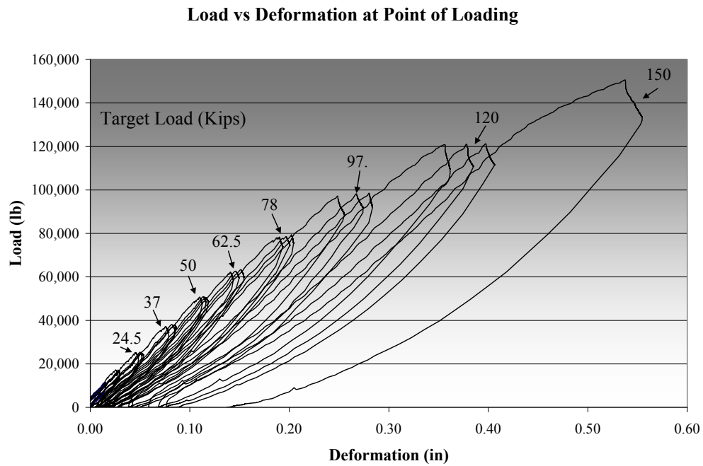
Figure 2.25: January cyclic load vs. deformation at point of load.
