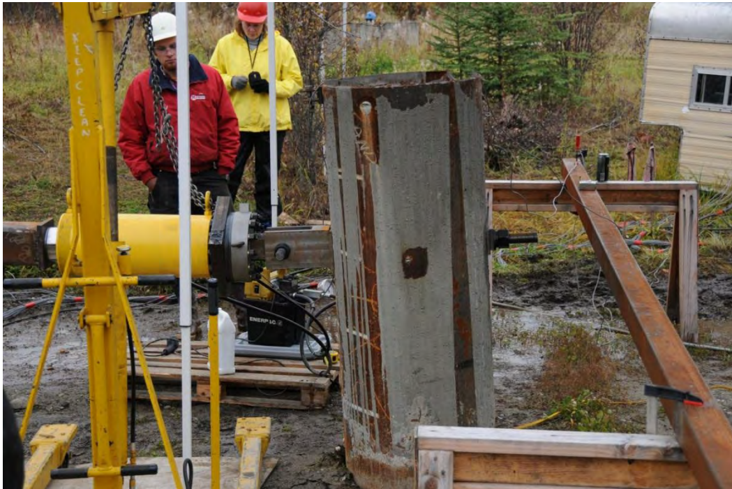
Figure 2.21: Reaction pile at final September load increment.
