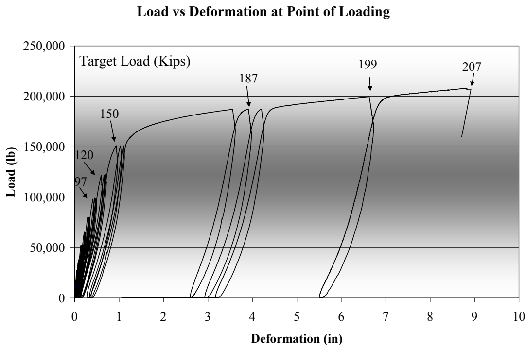
Figure 2.28: March cyclic load vs. deformation at point of load 0 to 207 kips.
