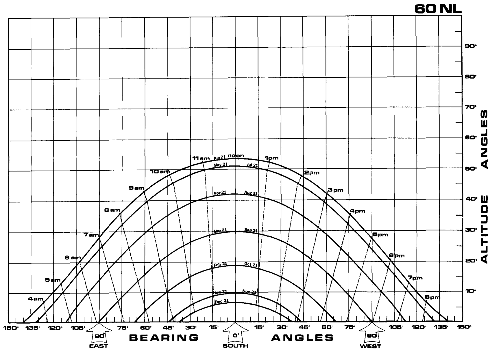
Figure 43. Sun path diagram for 60°N latitude.
