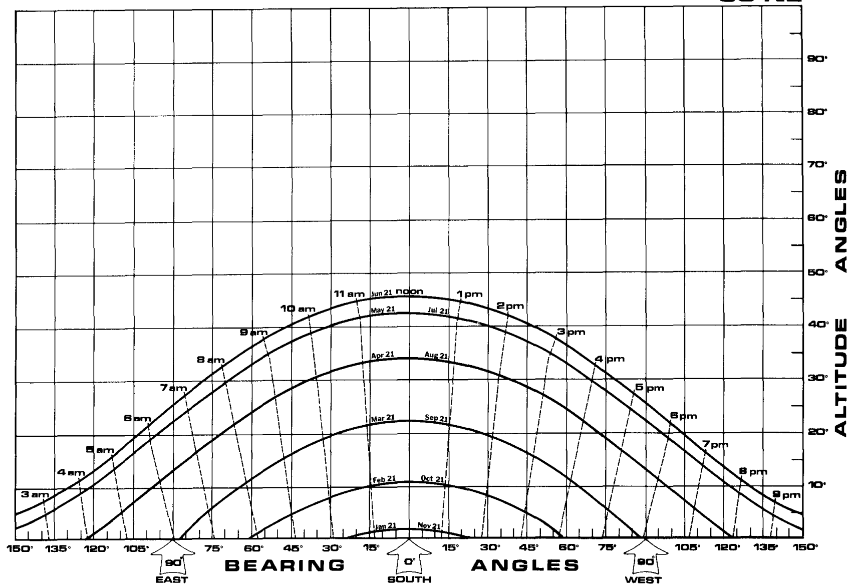
Figure 47. Sun path diagram for 68°N latitude.
