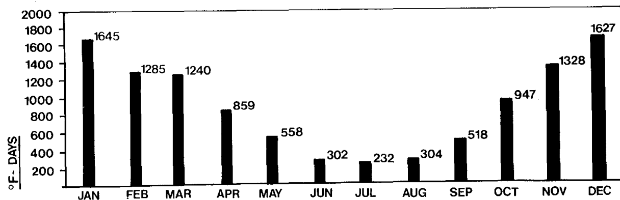
Average Monthly Heating Degree Days
