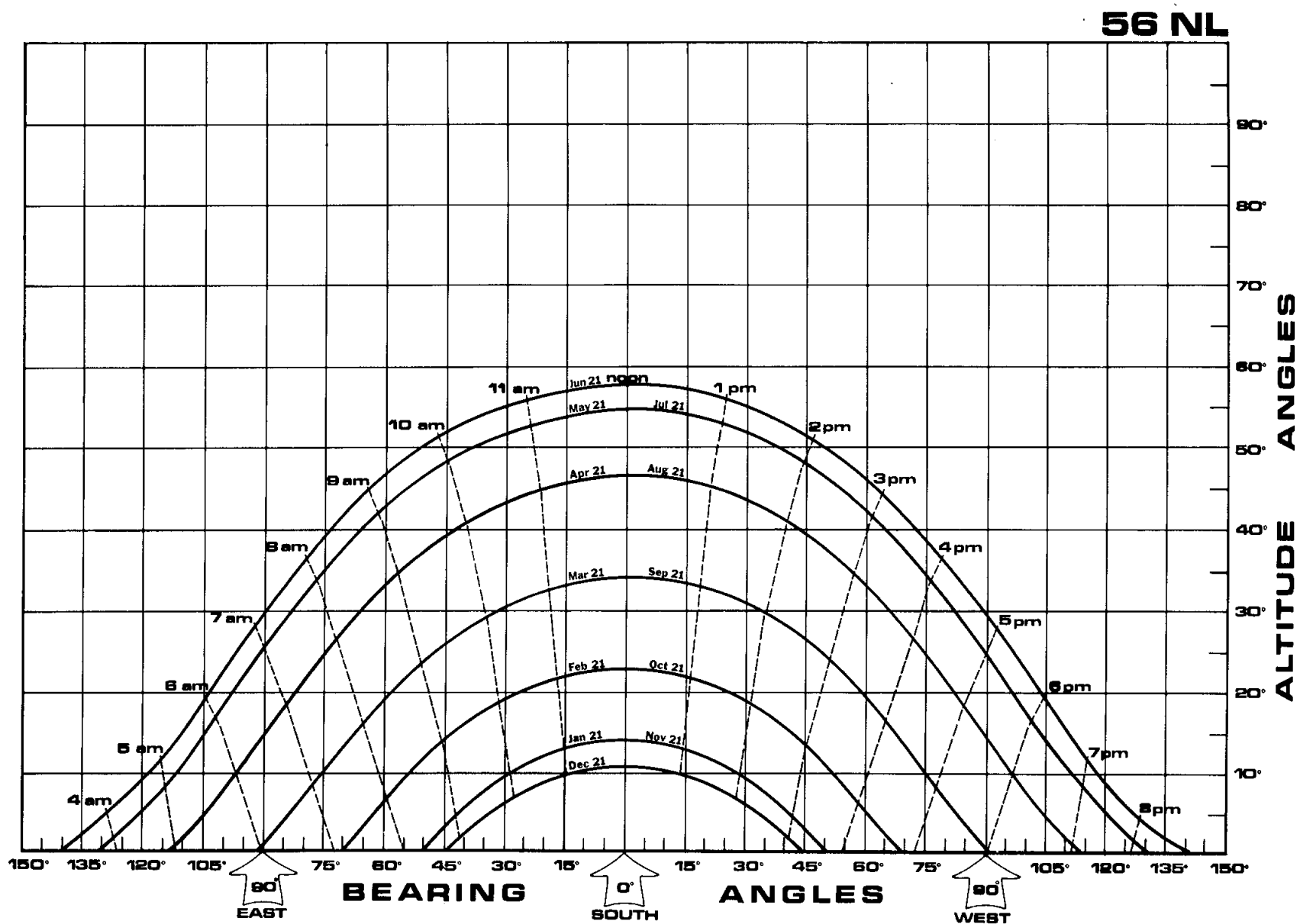
Figure 41. Sun path diagram for 56°N latitude.
