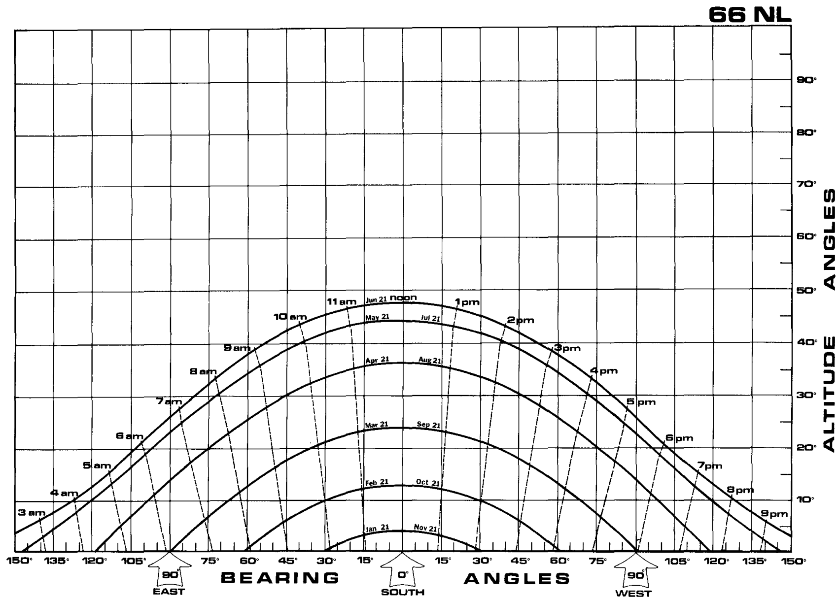
Figure 46. Sun path diagram for 66°N latitude.
