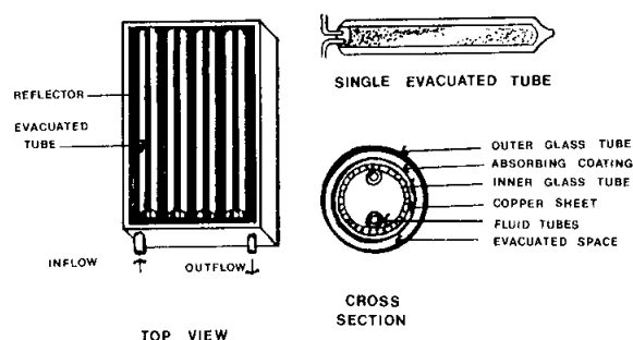
Figure 8. Various components of an evacuated-tube solar collector.
