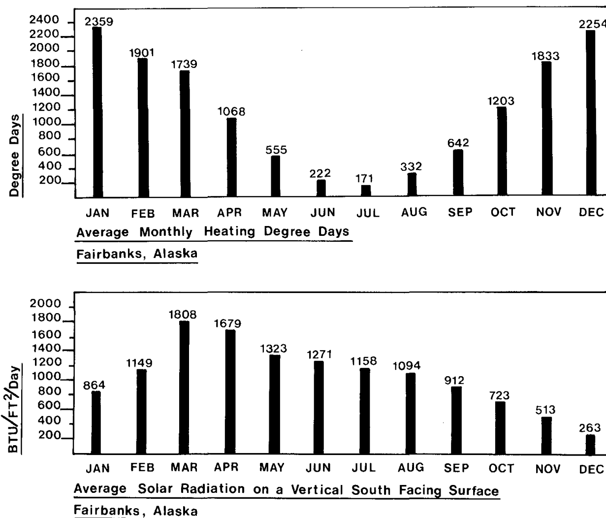
Figure 55. These graphs illustrate that the Fairbanks heating degree days and average solar radiation (which are an indication of a building's heating requirements) are not in phase with the solar radiation on a south-facing vertical surface. This has positive implications for passive solar heating. The solar gain is highest in March and April when heating is needed. Data are from Kusuda and Ishii (1977).
