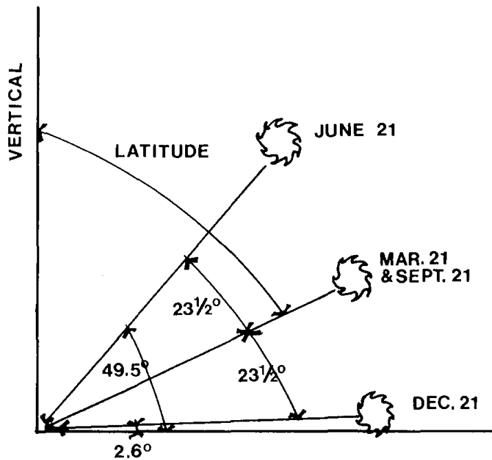
Figure 70a. The range of solar elevation angles at the latitude of Fairbanks (64°N). The maximum elevation is 49.5° on June 21, and the minimum is 2.6° on December 21.
