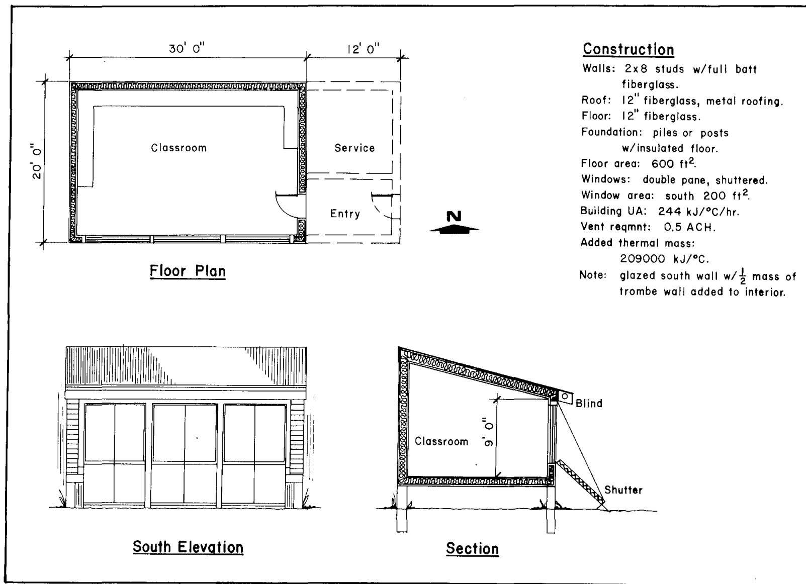
Figure 61. Design Test 5, a simple direct gain design with night insulation.
