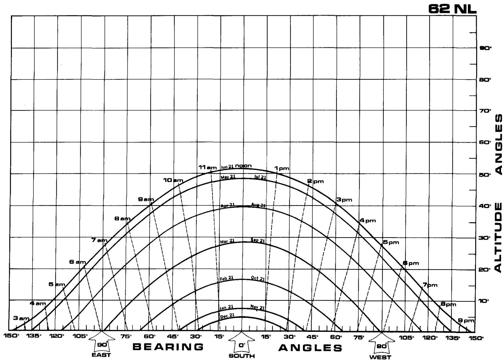
Figure 44. Sun path diagram for 62°N latitude.
