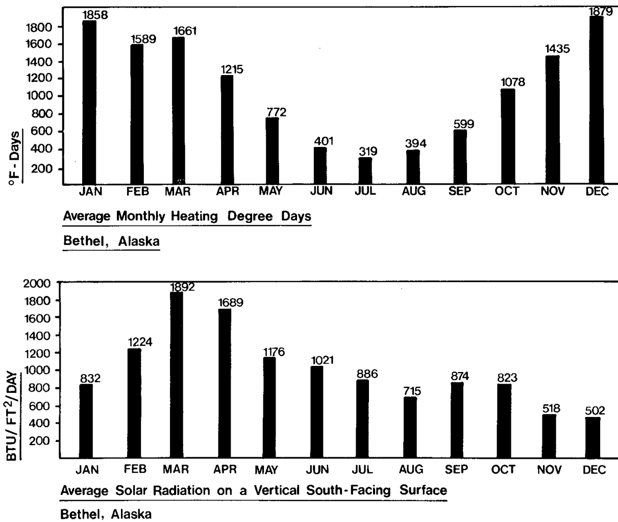
Figure 57. Bethel heating degree days and average solar radiation. These graphs illustrate that the annual heating degree days (which are an indication of a building's heating requirements) are not in phase with the solar radiation on a south-facing vertical surface. This has positive implications for passive solar heating. The solar gain is highest in March and April when heating is needed. Data are from Kusuda and Ishii (1977).
