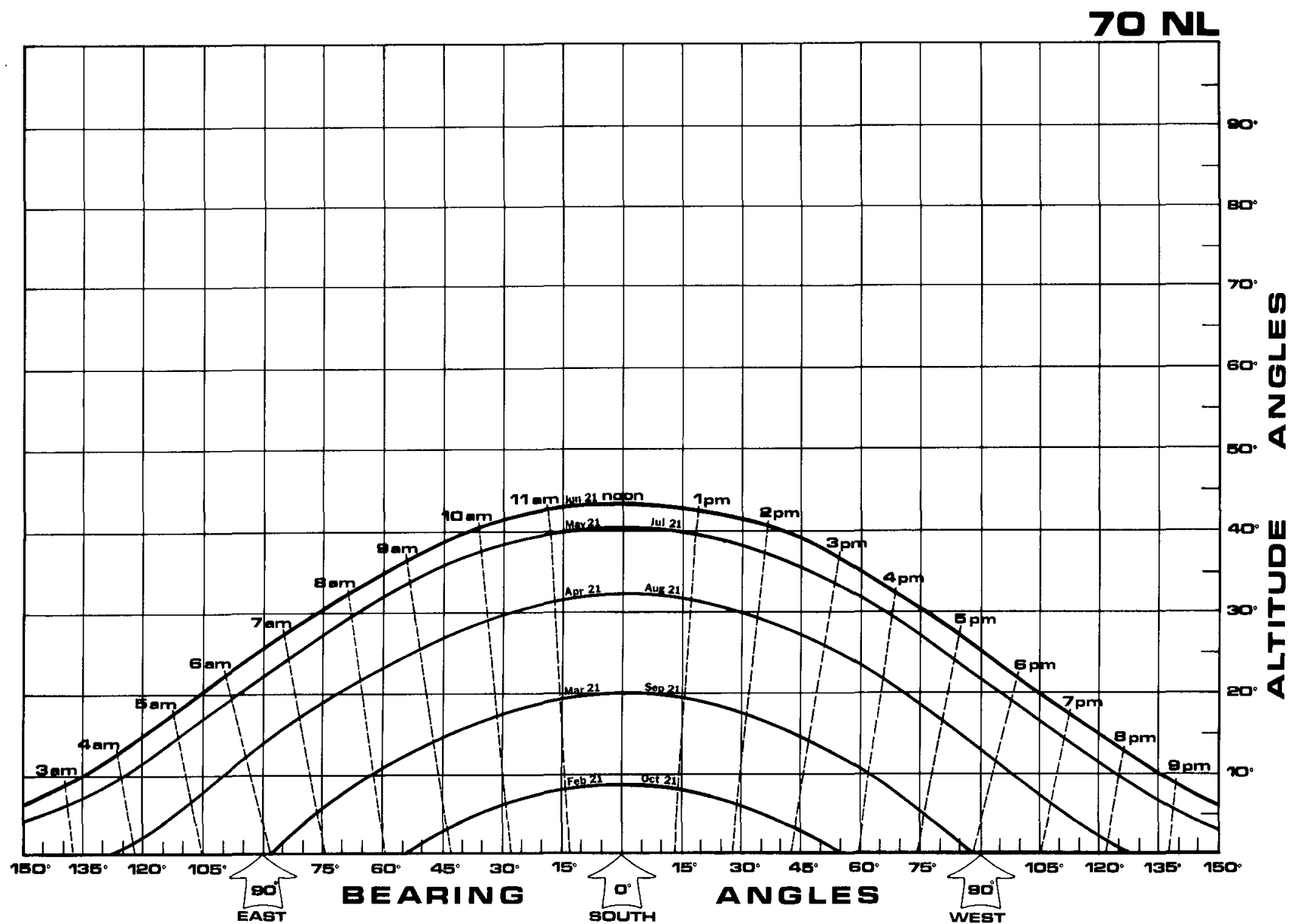
Figure 48. Sun path diagram for 70°N latitude.
