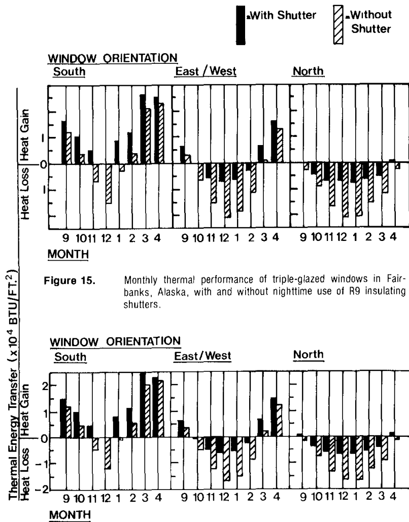
Figure 16. Monthly thermal performance of quadruple-glazed windows in Fairbanks, Alaska, with and without nighttime use of R9 insulating shutters.
