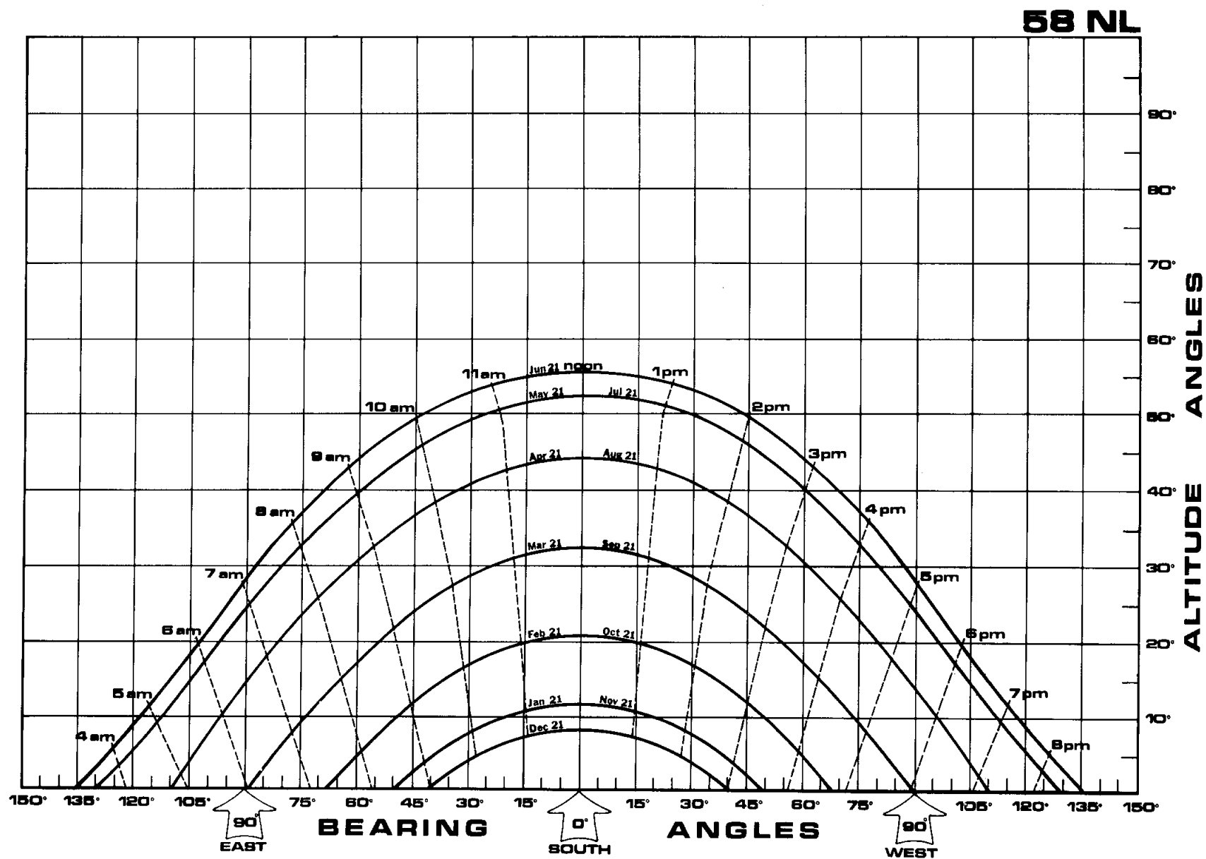
Figure 42. Sun path diagram for 58°N latitude.
