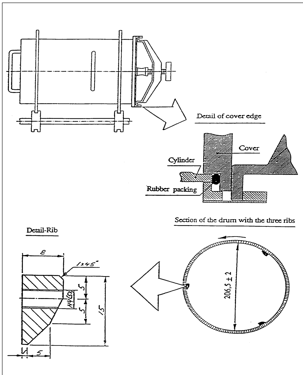
Figure 1 All Dimensions in mm
