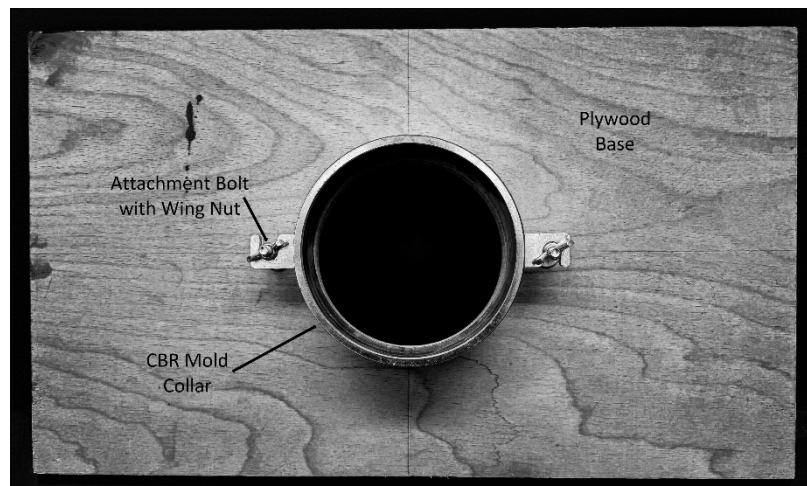
Figure 4. Abrader base plate guide for field abrasion
