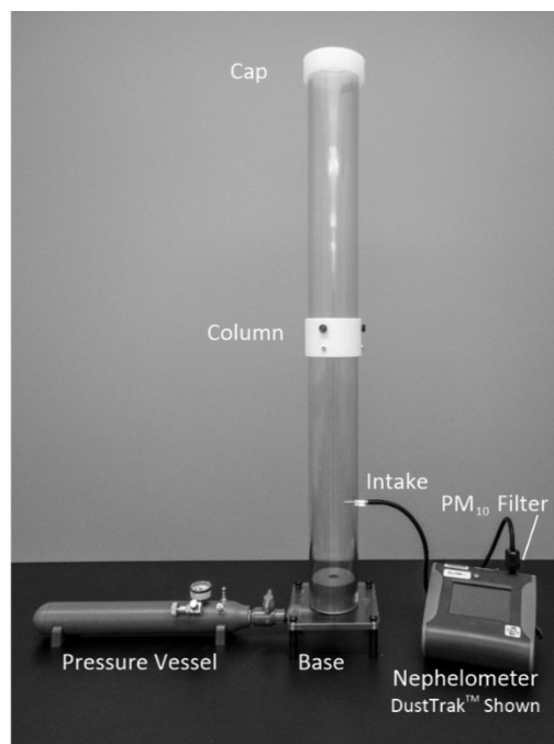
Figure 1. Column apparatus
