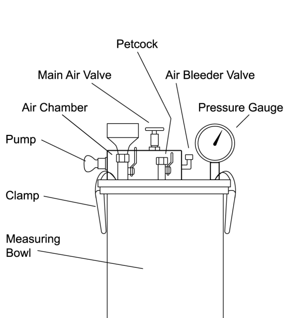
2a. Horizontal Air Chamber
