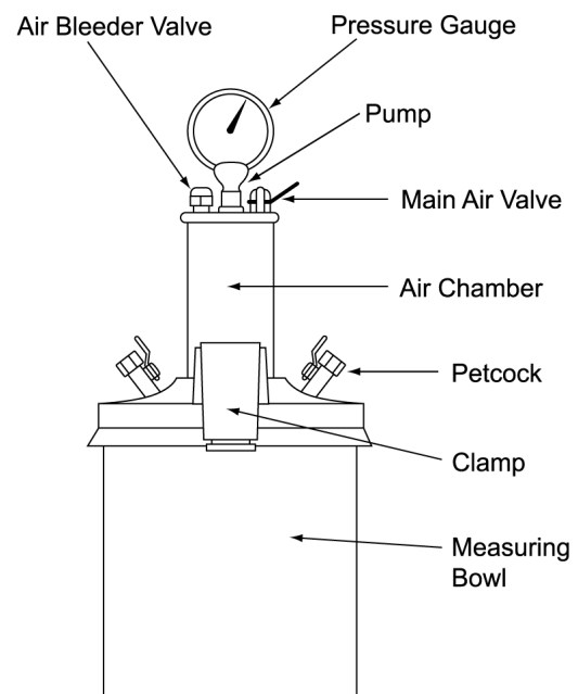
2b. Vertical Air Chamber
