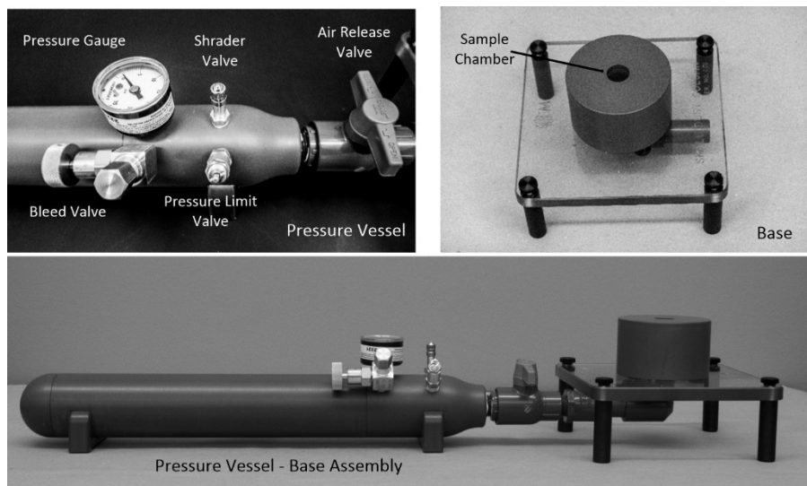
Figure 2. Pressure vessel and base assembly
