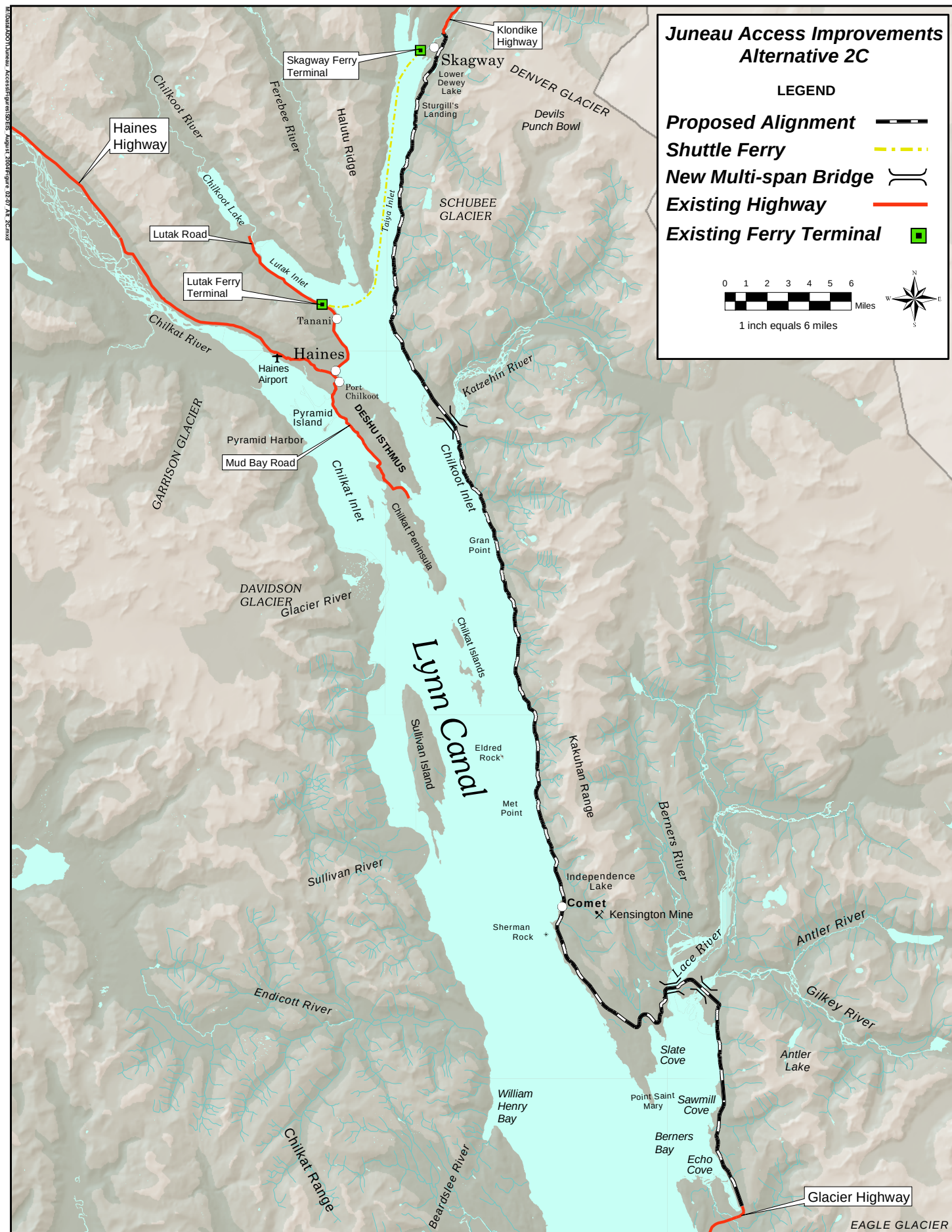
Figure 2-7 Alternative 2C: East Lynn Canal Highway with Haines/Skagway Shuttle
