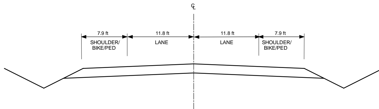
TYPICAL ROADWAY SECTION NTS
