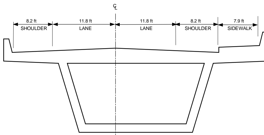
TYPICAL BRIDGE SECTION NTS
