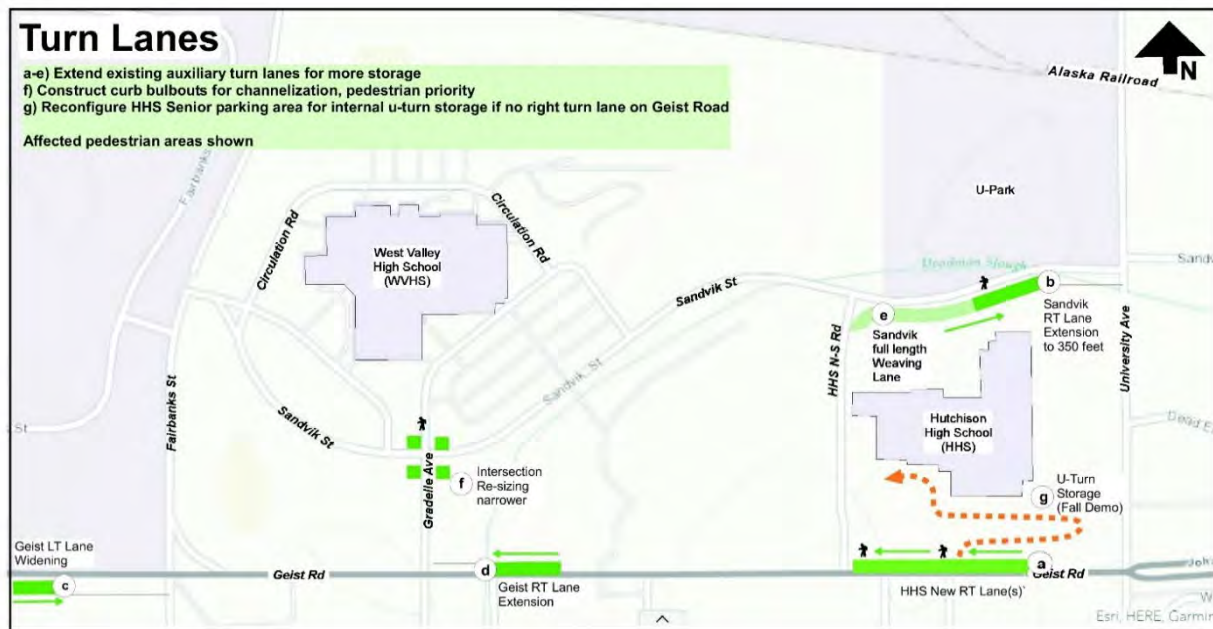
Figure 8. Extended Turn Lane Options
