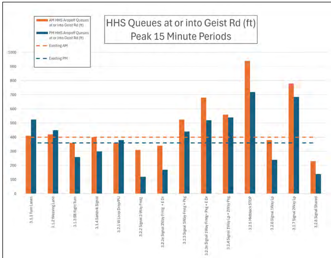
Figure 60. HHS Queues at or onto Geist Road across Options
