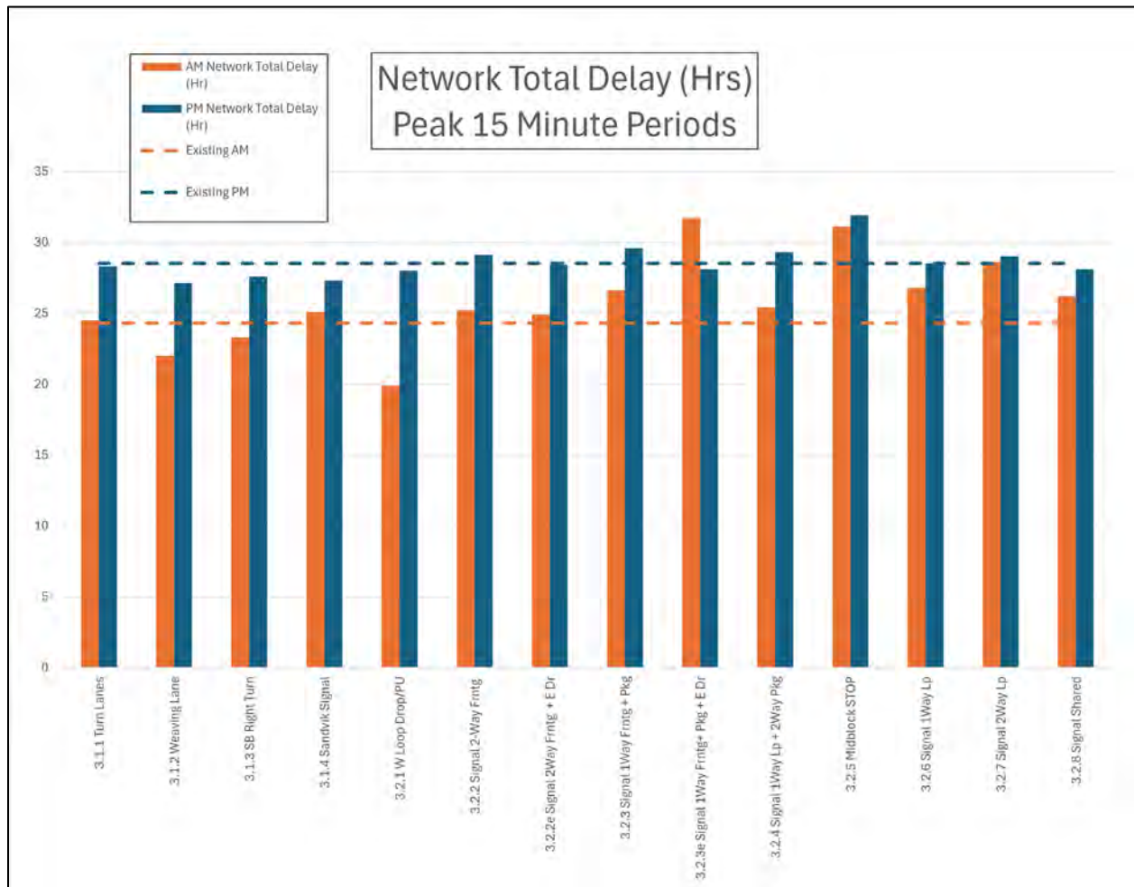
Figure 54. Comparison of Total Network Delay across Options
