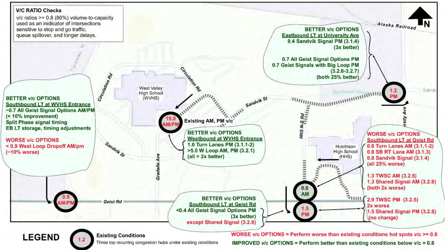
Figure 62. Locations with v/c ratios of concern for existing conditions and analysis options
