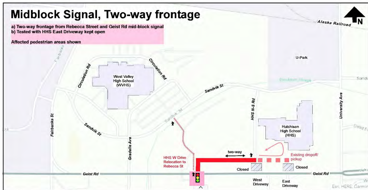
Figure 25. Signal, Midblock, Two-way frontage option (HHS)
