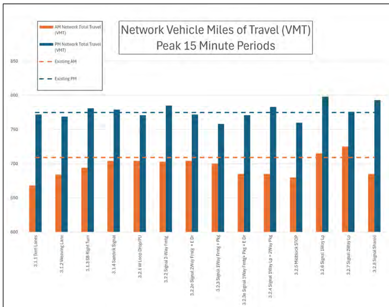
Figure 56. Comparison of Vehicle Miles of Travel across Options
