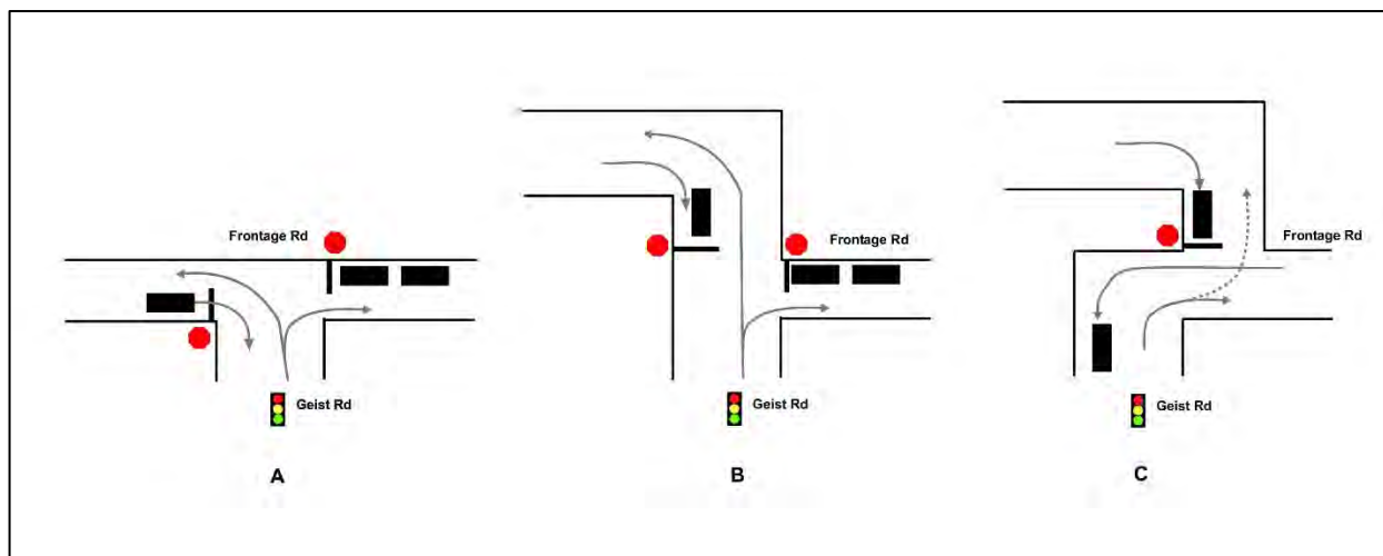
Figure 63. Offset tee model options for a midblock signal on Geist Road
