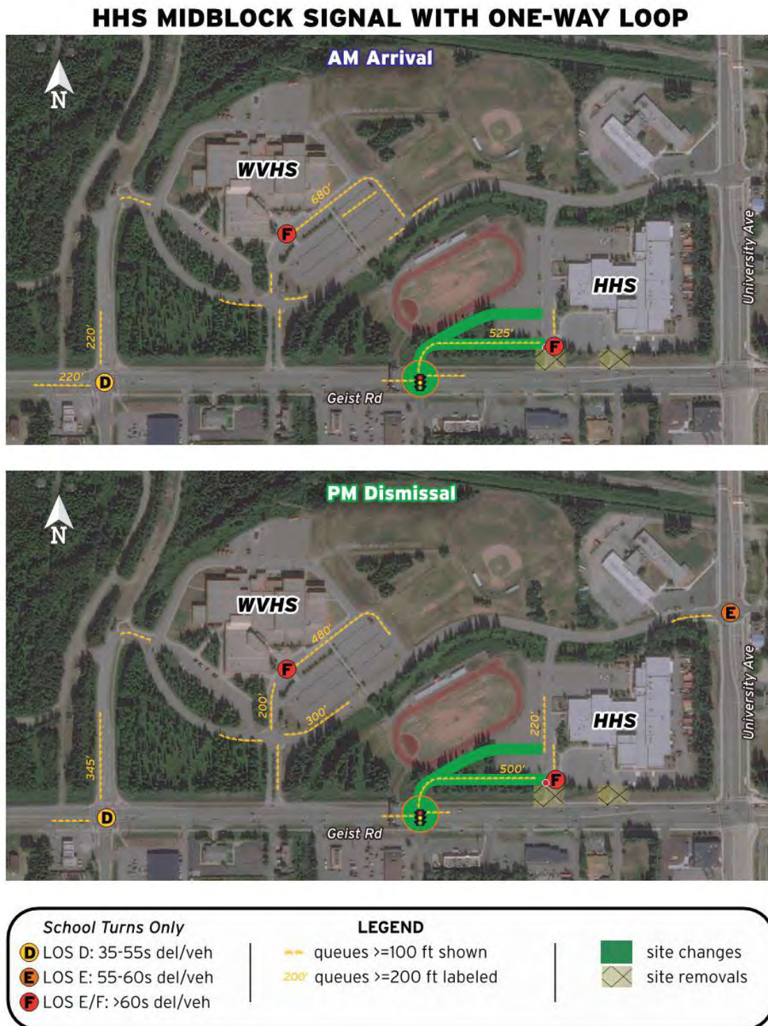
Figure 28. Midblock Signal, Short One-way Frontage Loop Performance Map
