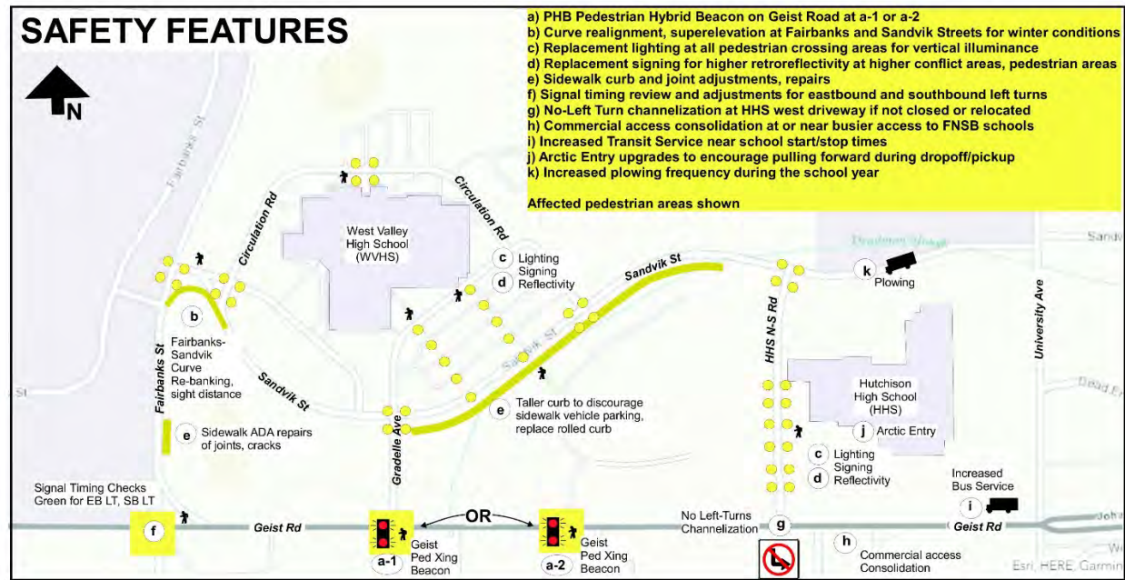
Figure 39. Safety and Operational Improvement Options
