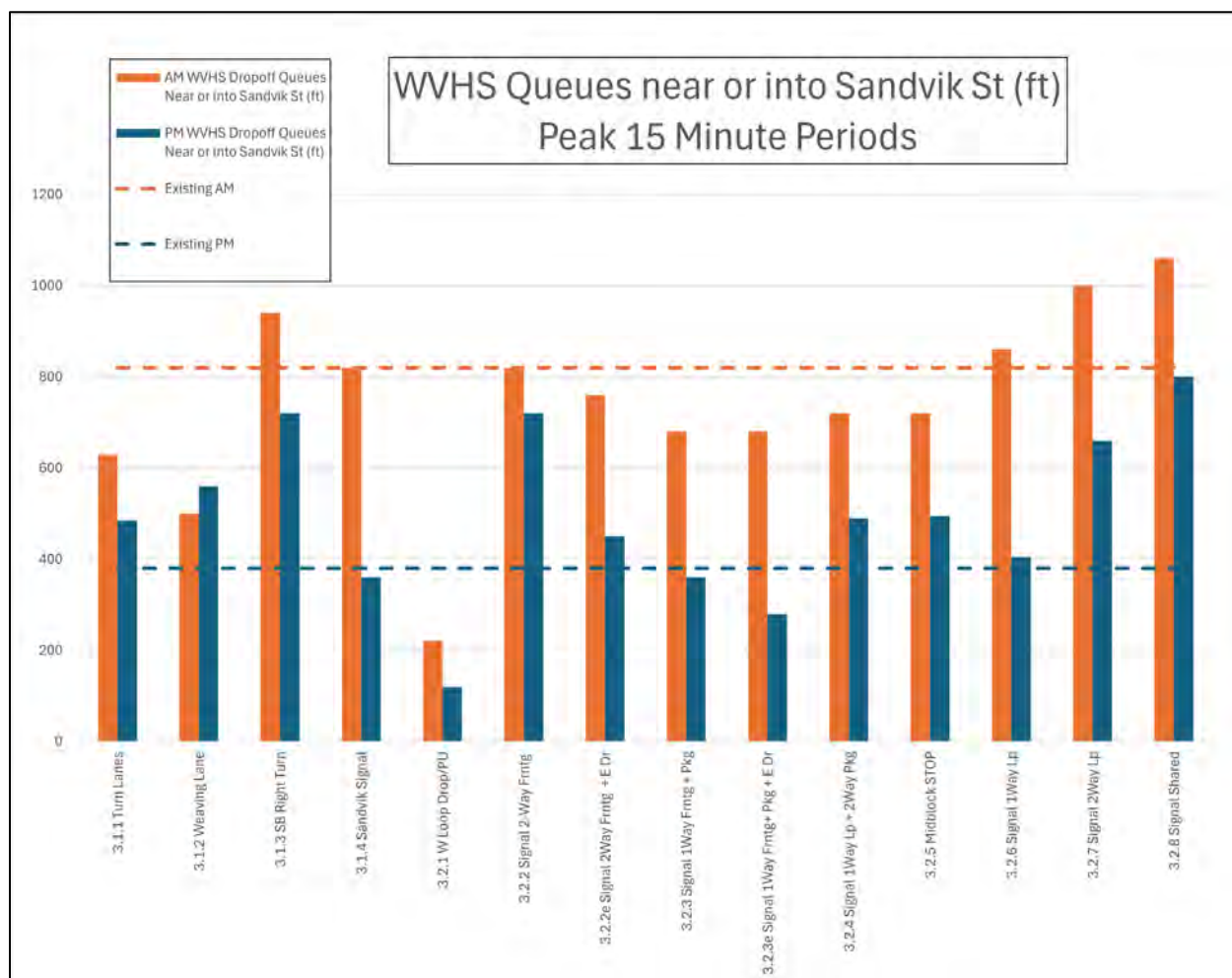
Figure 58. WVHS Queues near or into Sandvik St across Options
