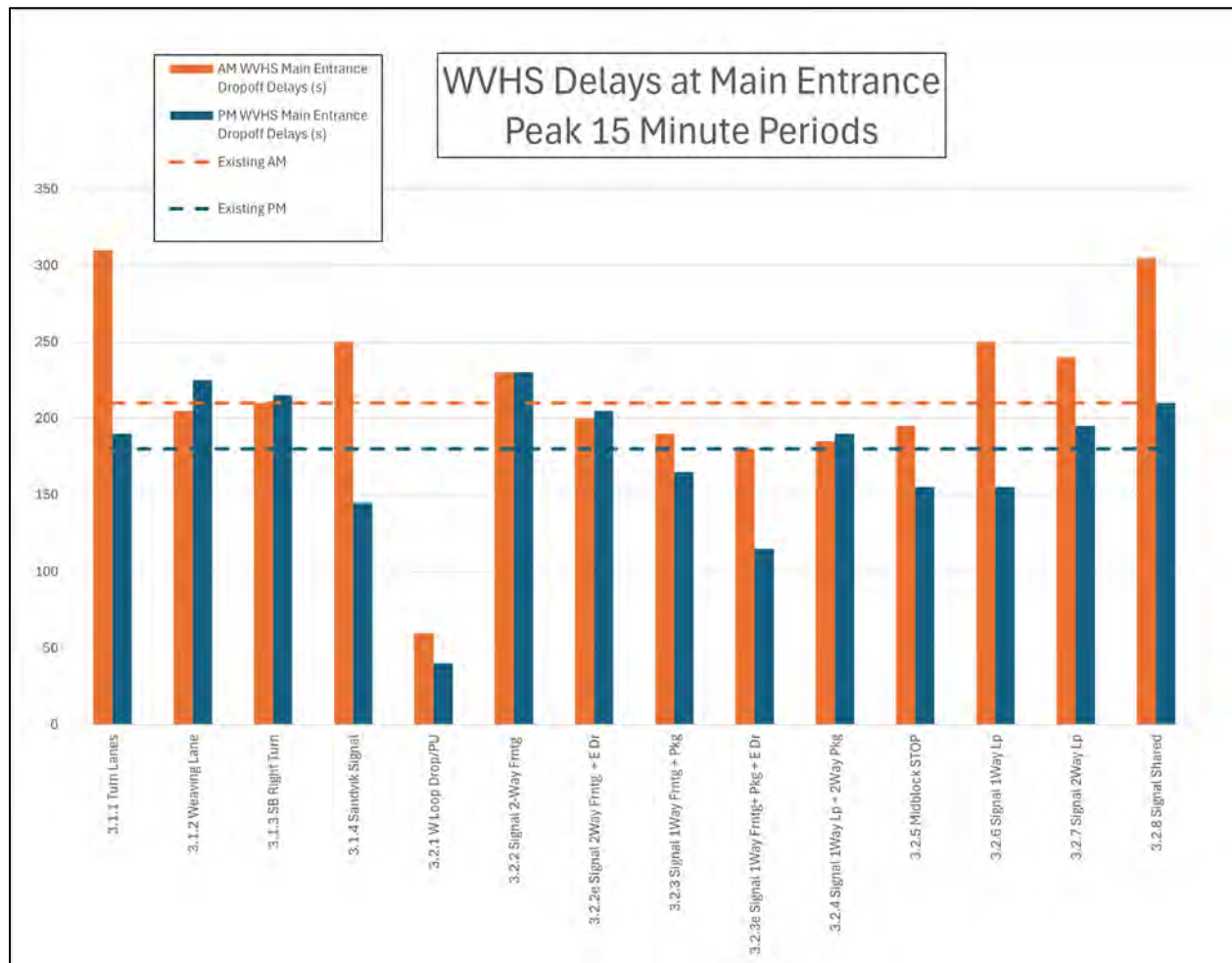
Figure 59. WVHS Delays at Main Entrance across Options
