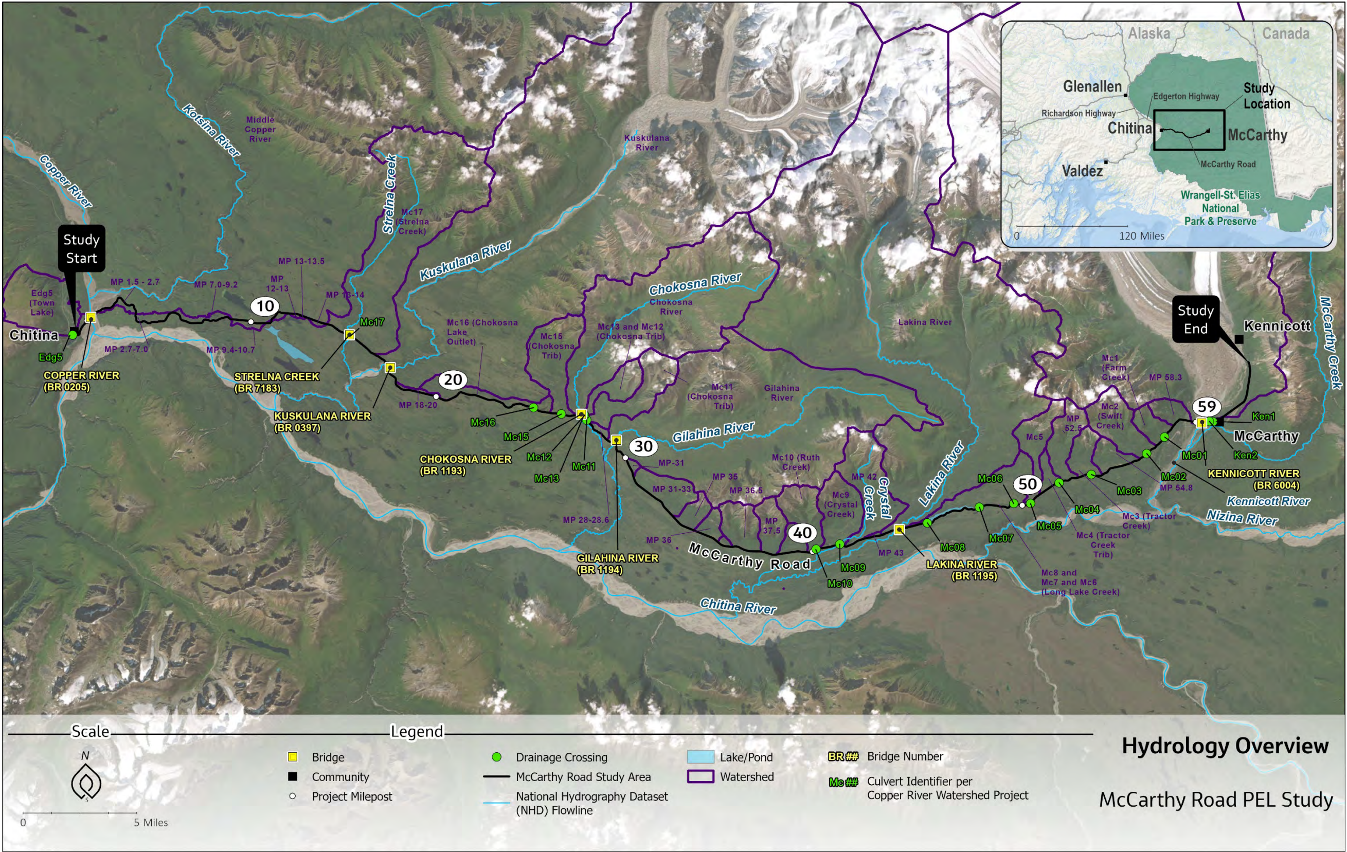
Figure 6-39. Hydrology Overview
