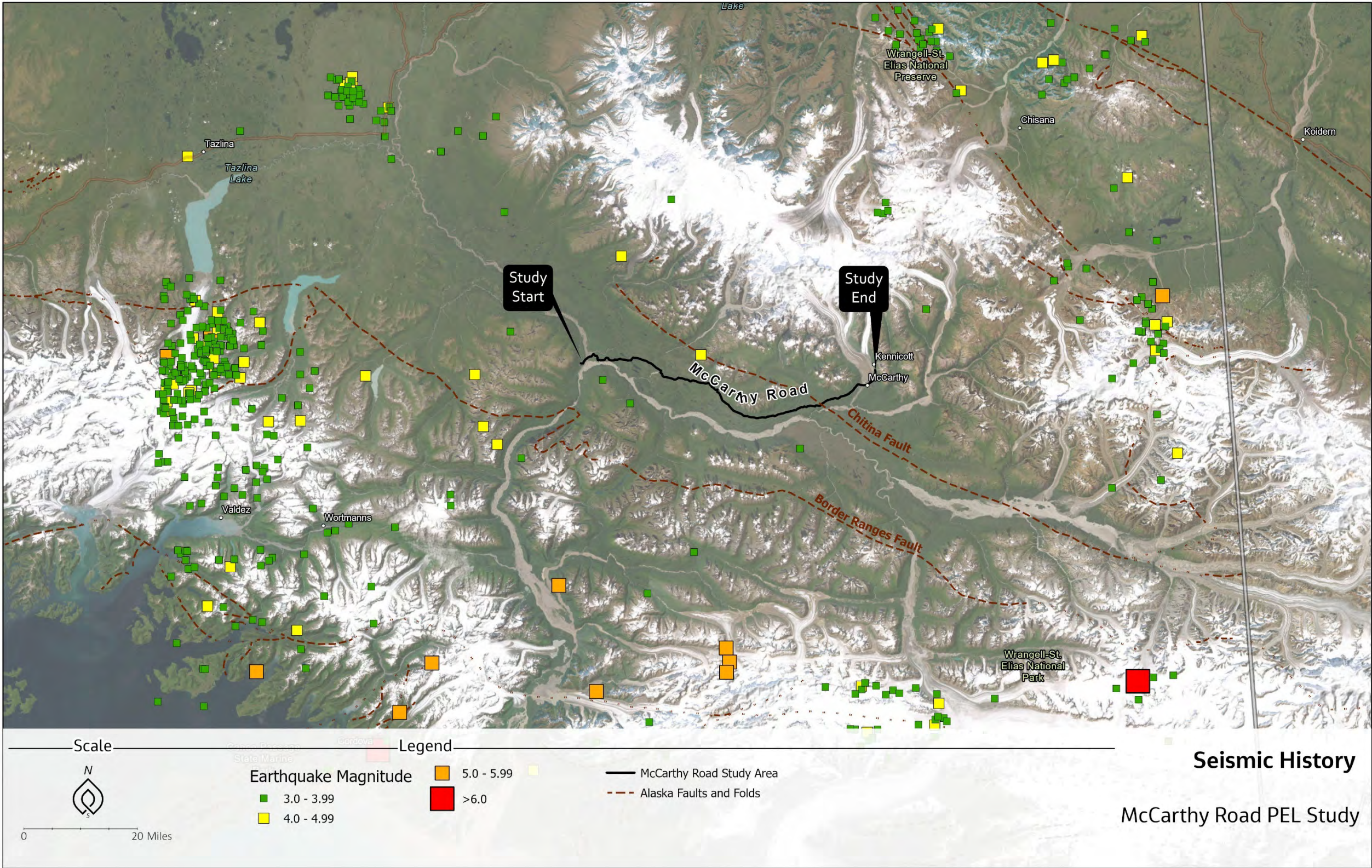
Figure 7-2. Historical Seismicity and Faulting
