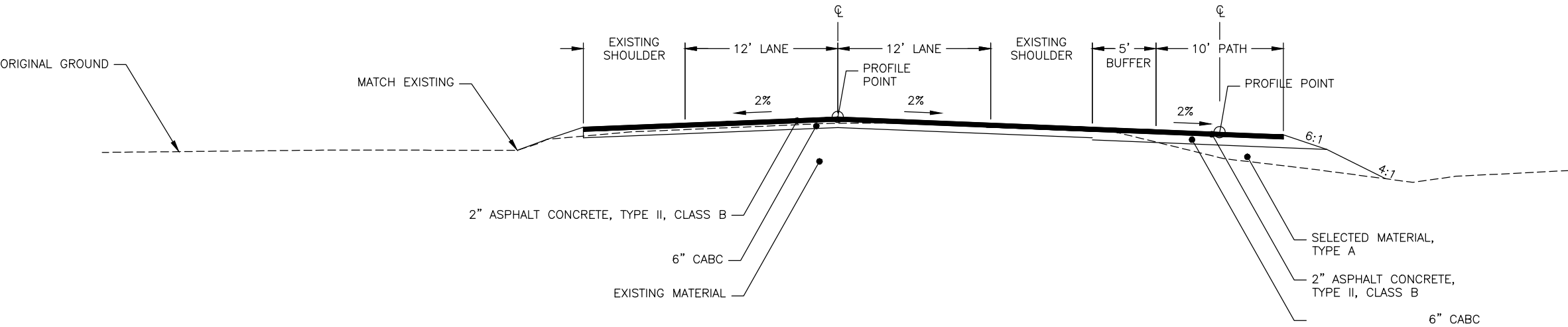
AIRPORT WAY ATTACHED PATH SECTION 3
