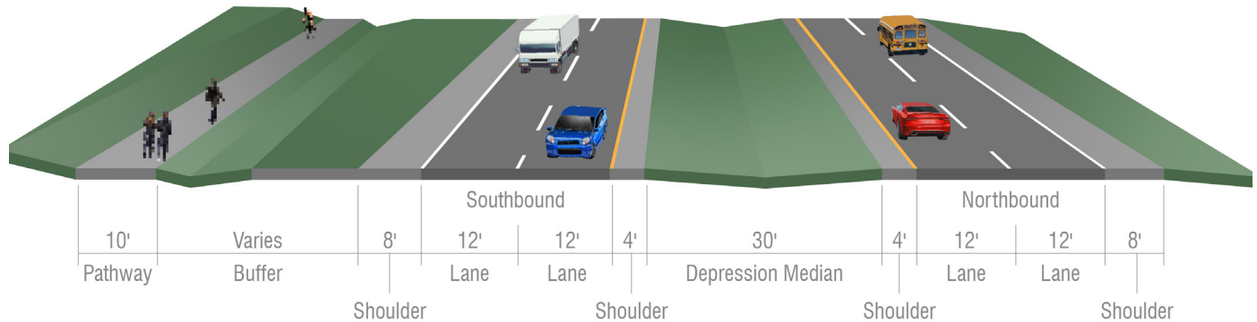
Figure 1: Typical Section
