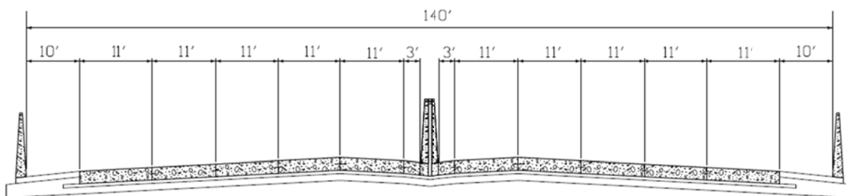
Figure 59. Case Study 5, Alternative 2 Typical Section
