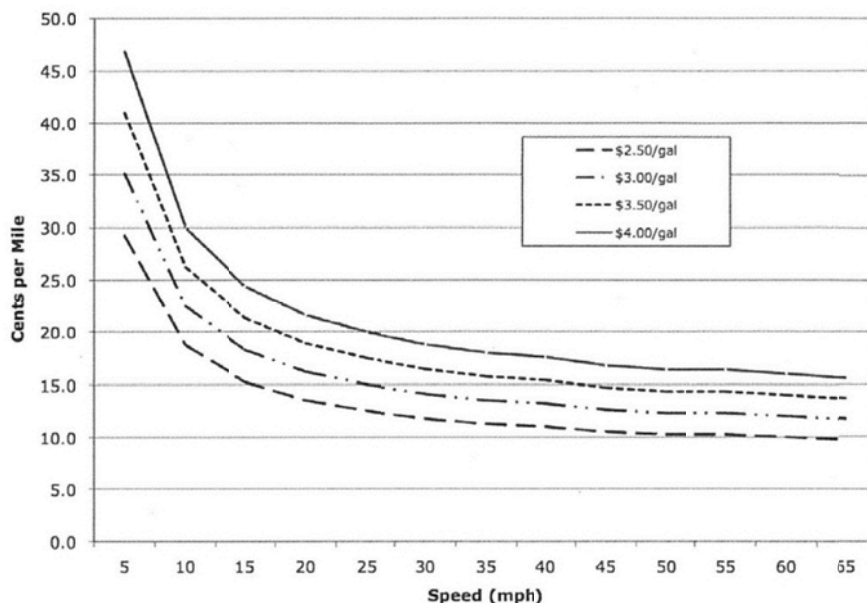
Figure 34. Fuel Costs (Cents per Mile) by Speed – Automobiles ref figure 5-1 User Benefit Analysis for Highways AASHTO 2003
