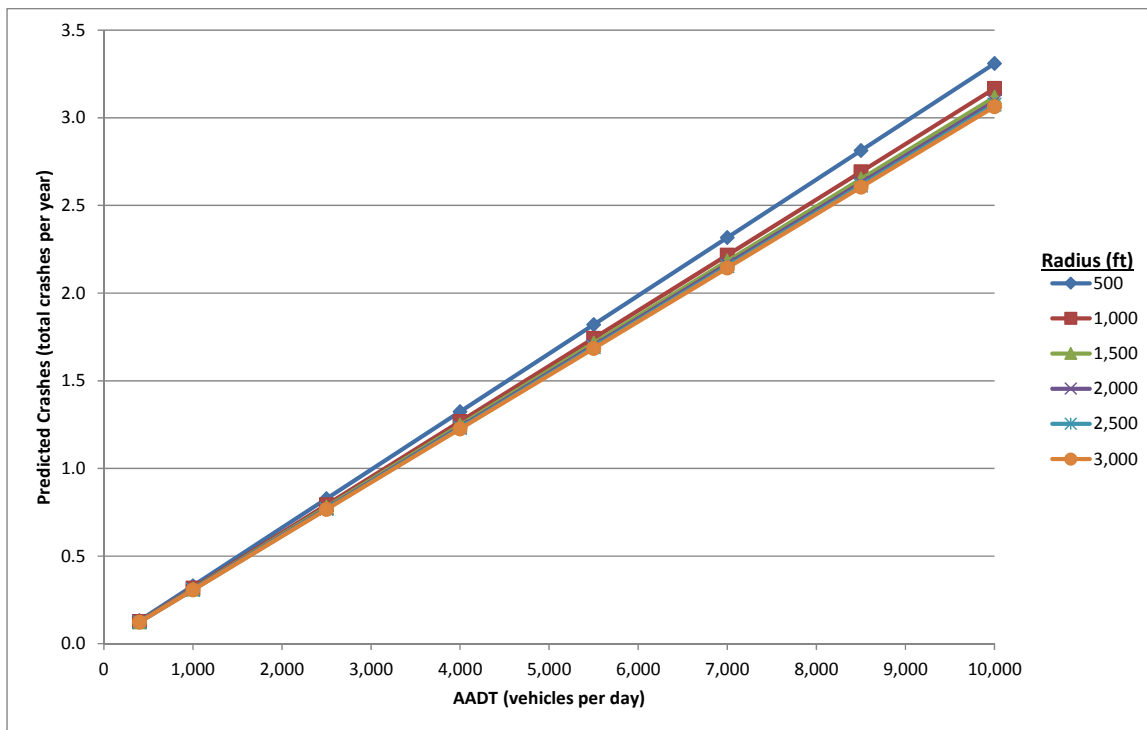
Figure C-3. Annual Predicted Crash Frequency by Radius for a 30° Deflection Angle
