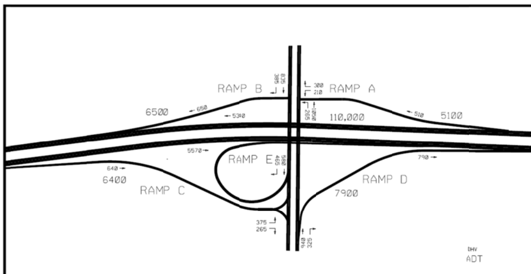
Figure 52. Design year peak hour turning movement counts for planned interchange reconfiguration.
