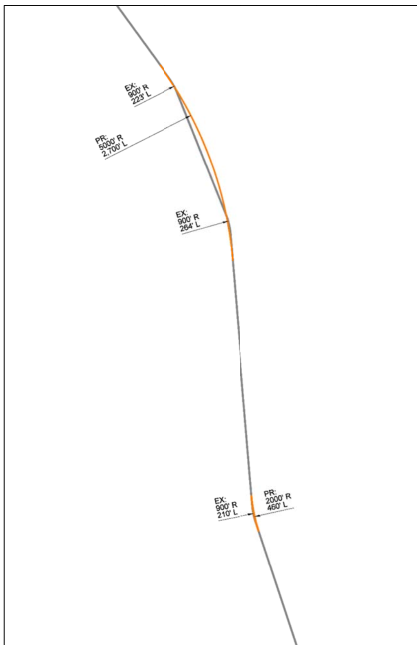
Figure 54. Two horizontal curves with existing and proposed alignments
