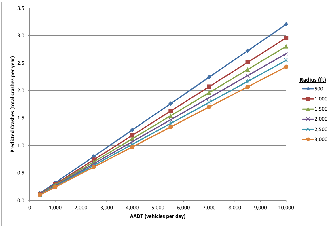
Figure C- 7. Annual Predicted Crash Frequency by Radius for a 90° Deflection Angle
