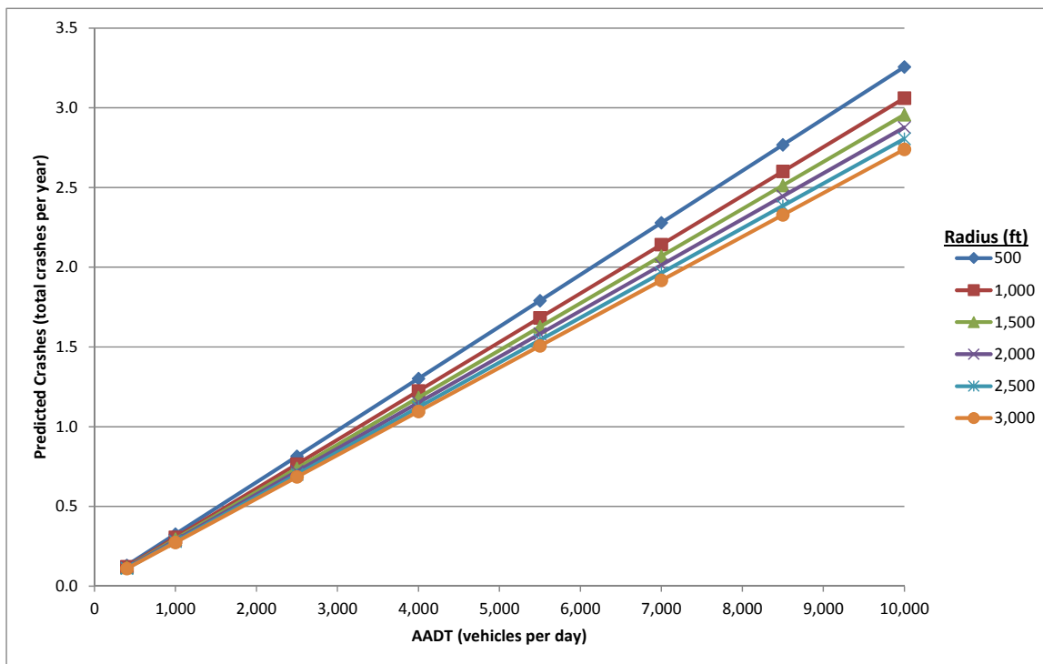
Figure C- 6. Annual Predicted Crash Frequency by Radius for a 75° Deflection Angle
