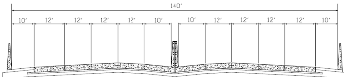
Figure 58. Case Study 5, Alternative 1 Typical Section
