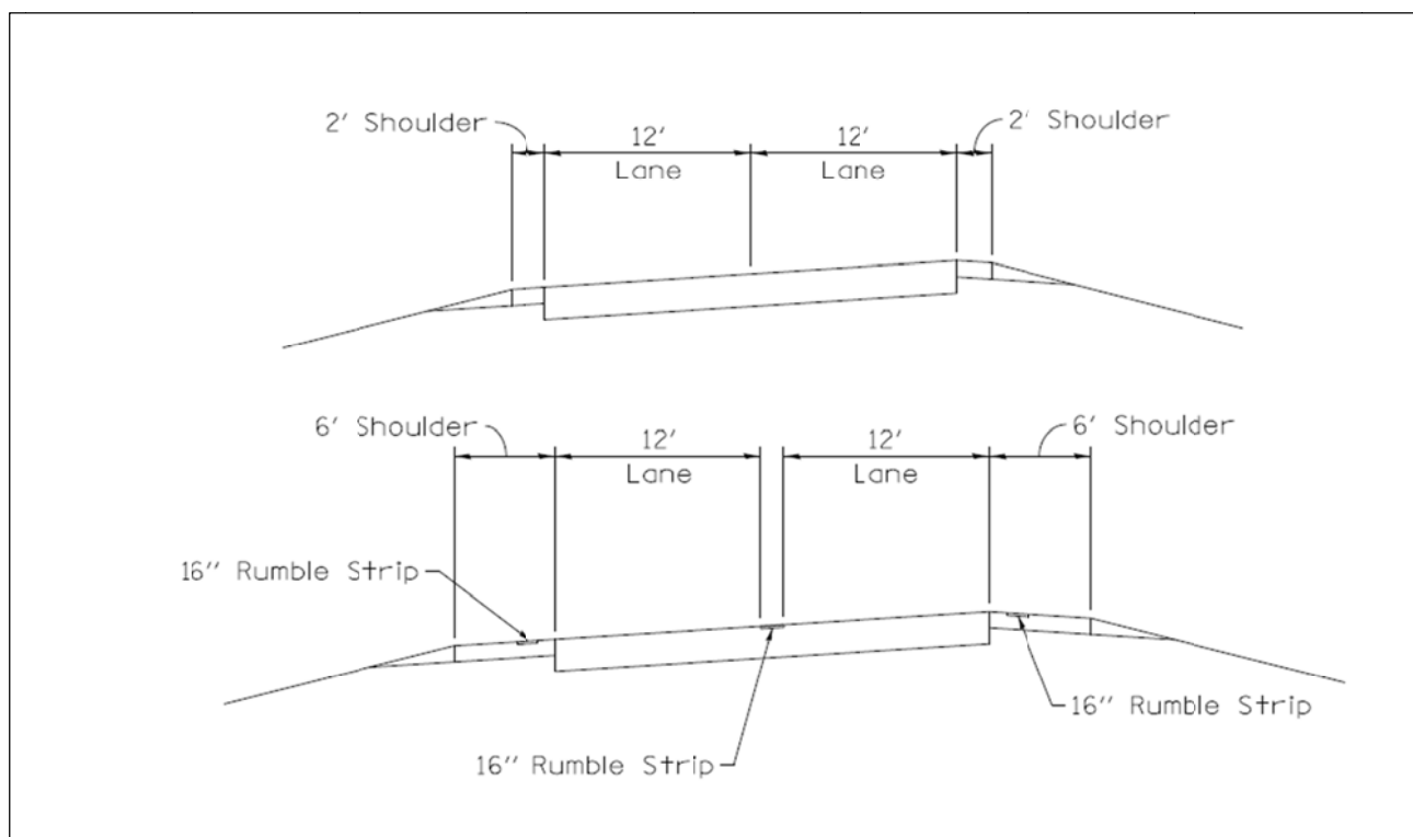
Figure 53. Cross-section before 3R improvement (top) and cross-section with improvement (bottom)
