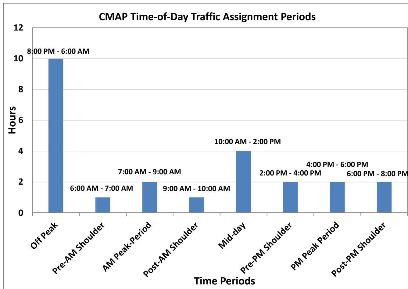
Figure 30. Traffic Assignment Periods Employed by the Chicago Metropolitan Agency of Planning (CMAP)
