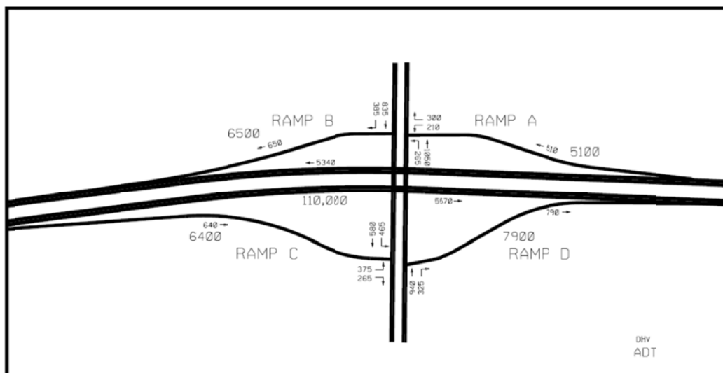
Figure 51. Design year traffic volumes for existing interchange configuration.
