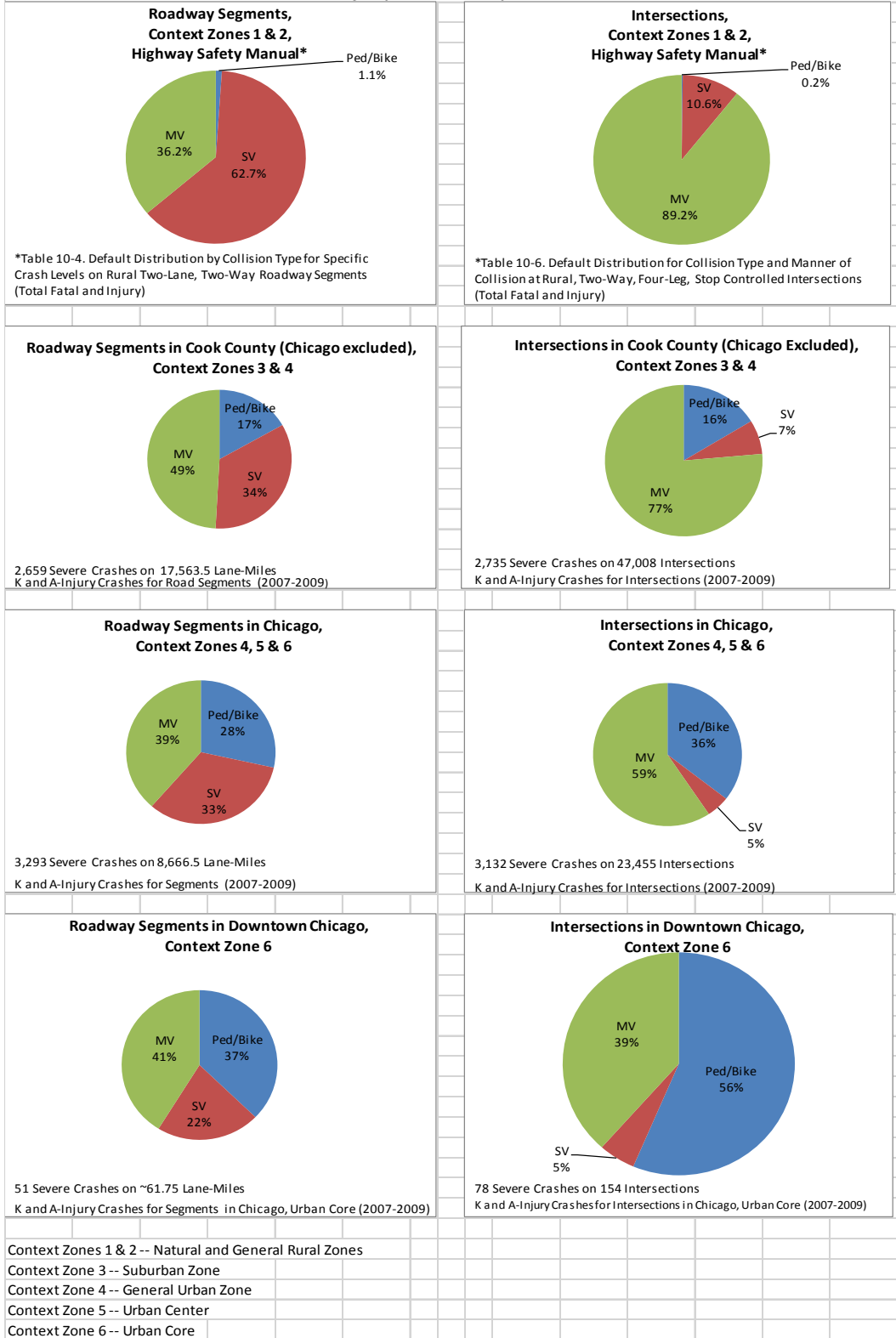
Figure 27. Profile of Fatal and Injury Crashes by Type for ITE Context Zones for Cook County IL
