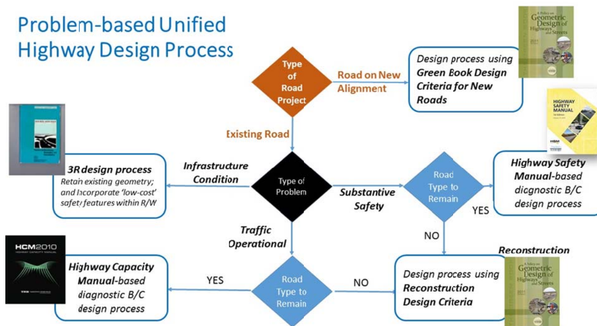
Figure 33. Problem-based Unified Geometric Design Process
