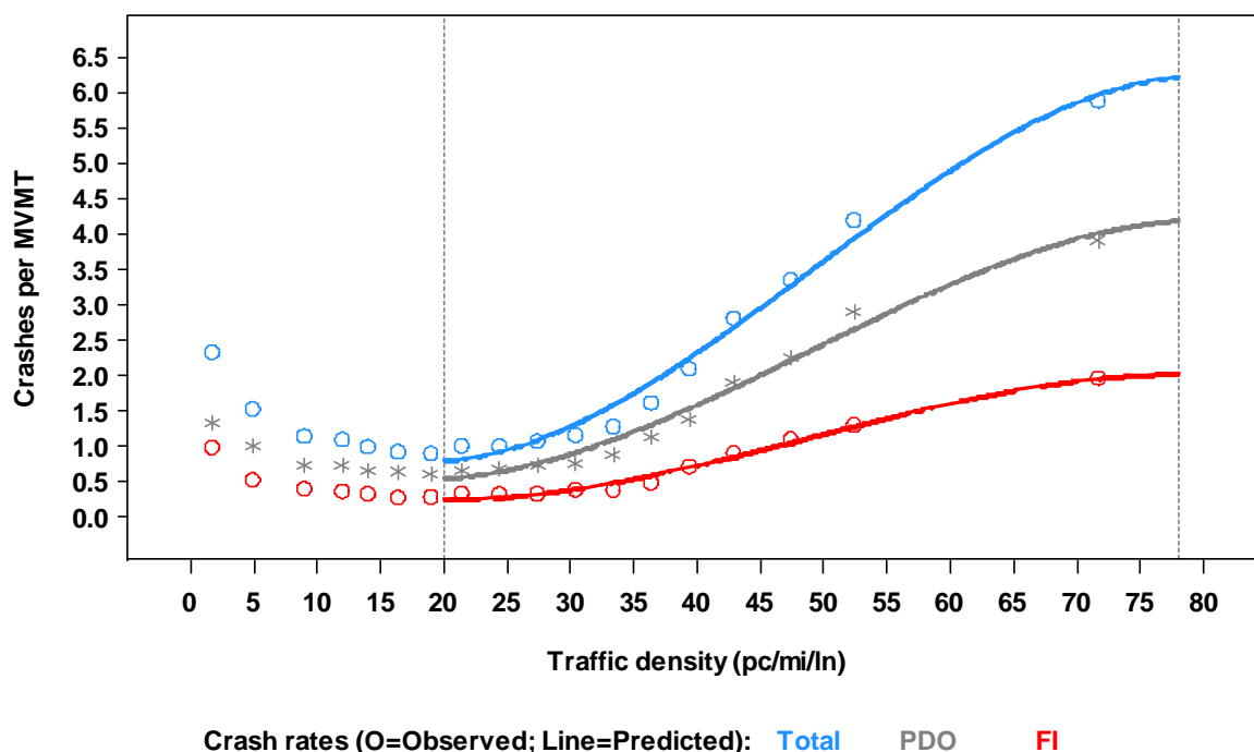
Figure 2. Typical Observed and Predicted Total, FI, and PDO Crash Rates vs. Traffic Density (ref to L07 report)
