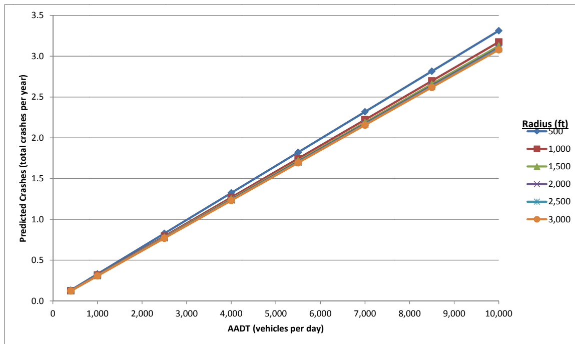
Figure C- 2. Annual Predicted Crash Frequency by Radius for a 15° Deflection Angle
