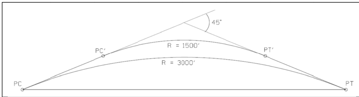
Figure C- 1. Comparison of Travel Distance with Same Central Angle
