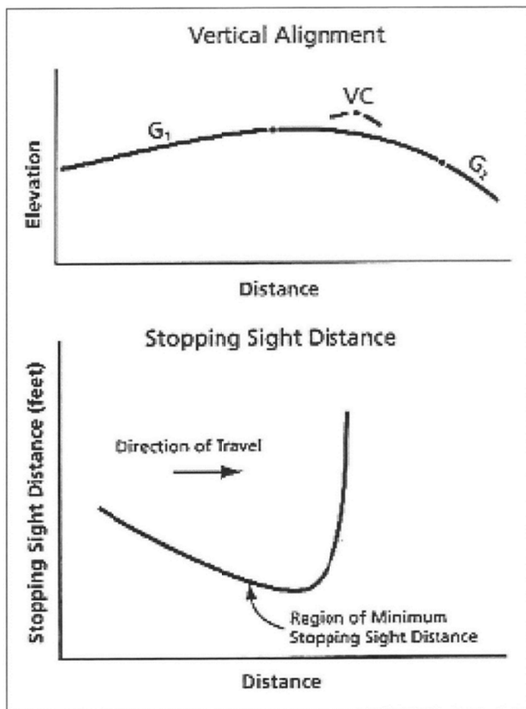
Figure 47. Stopping Sight Distance Profiles
