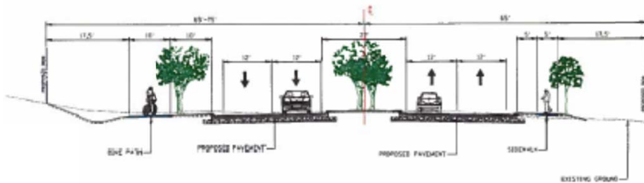
Figure 57. Proposed typical cross section for proposed alignment of highway (bypass).
