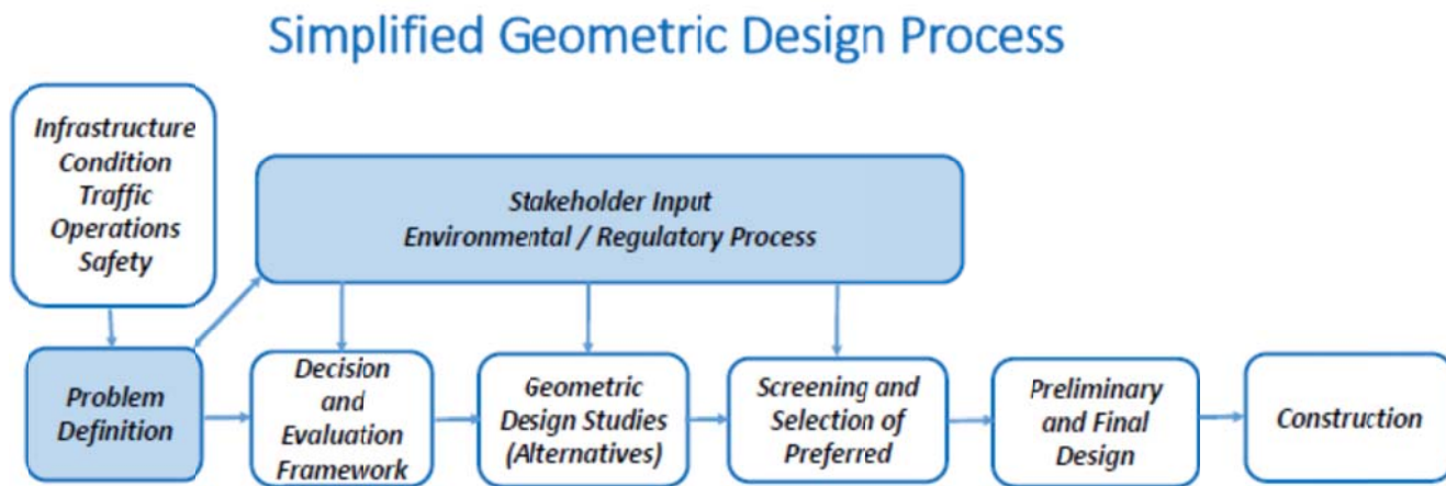
Figure 22. Roadway Design Development Process
