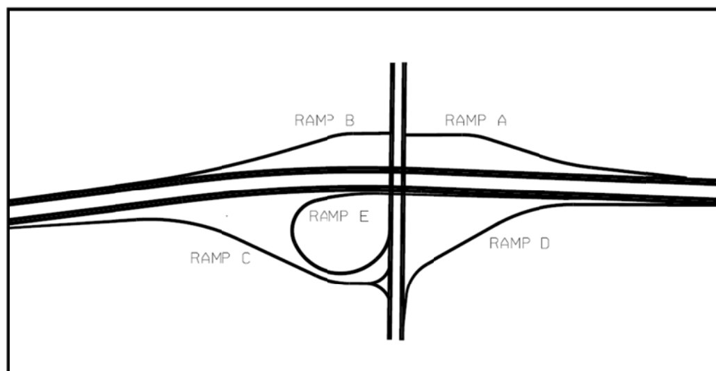
Figure 50. Proposed redesign of interchange, including new entrance loop ramp in southwest quadrant.
