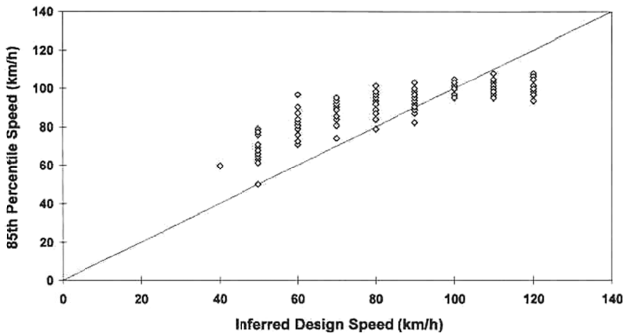
Figure 6. Comparison of Actual vs Assumed Driver Speed Behavior by AASHTO Curve Design Model
