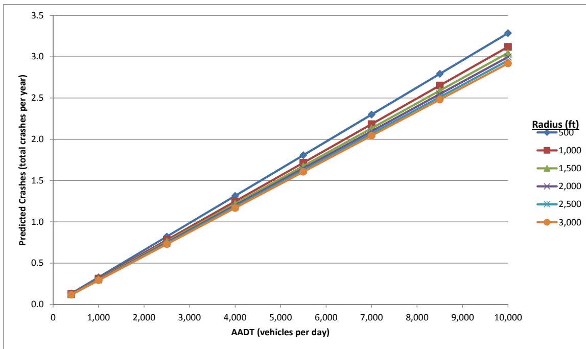
Figure C- 5. Annual Predicted Crash Frequency by Radius for a 60° Deflection Angle
