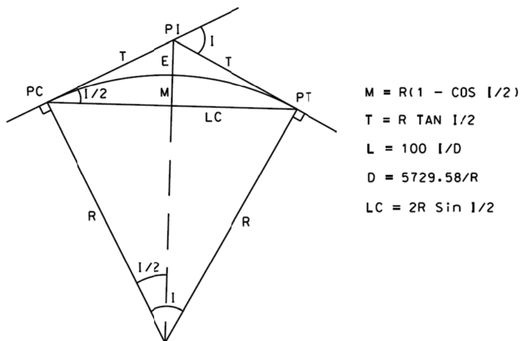
Figure 42. Curve Geometry
