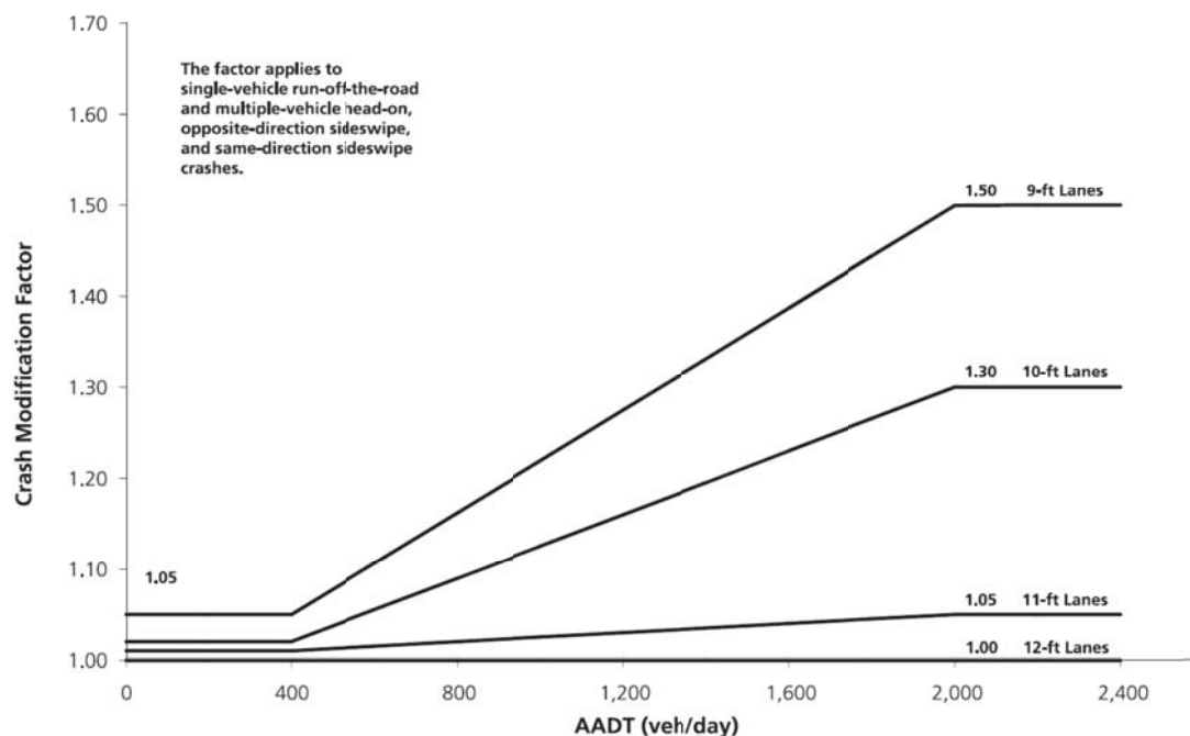
Figure 1. Crash Modification Factor for Lane Width on Roadway Segments
