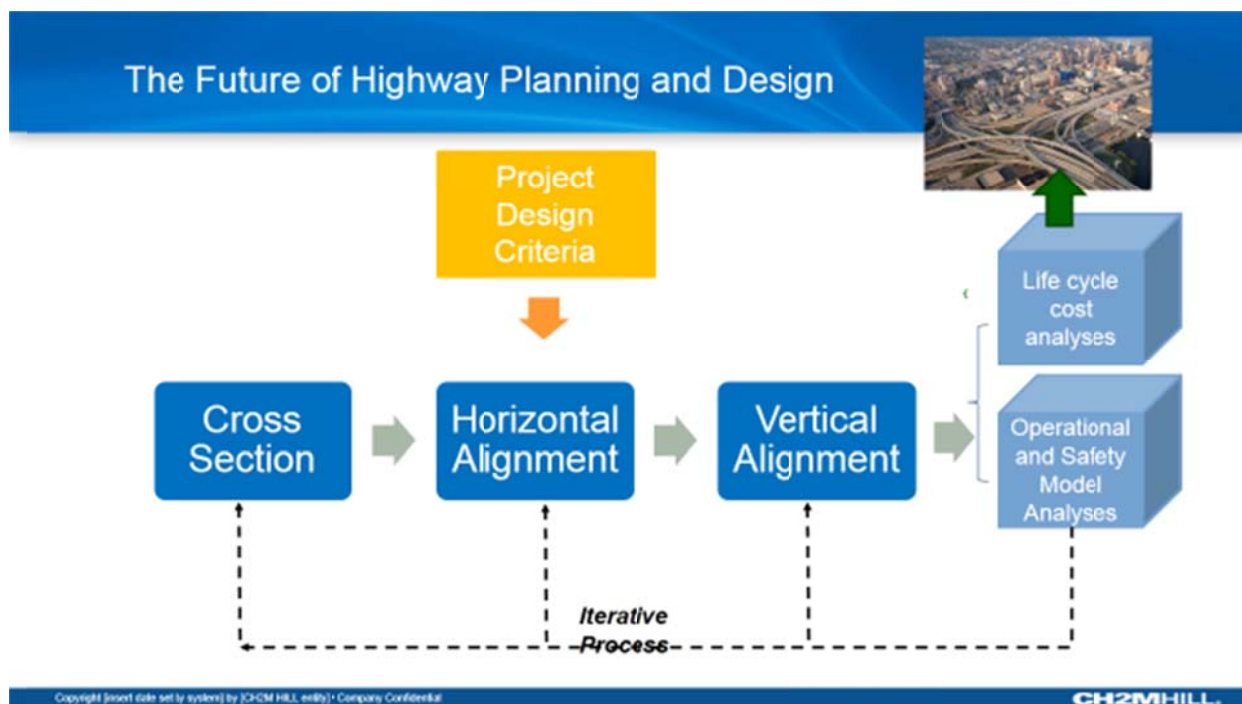
Figure 14. A Performance-based, Iterative Design Process
