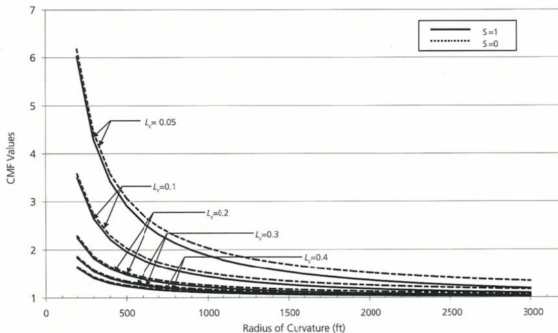
Figure 43. Potential Crash Effect of the Radius, Length, and Presence of Spiral Transition Curves in a Horizontal Curve
