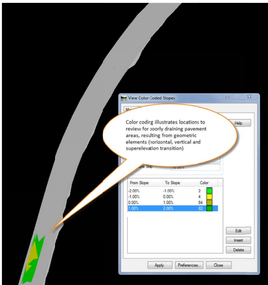
Figure 40. BIM Output to Evaluate Vertical Alignment Design for Drainage
