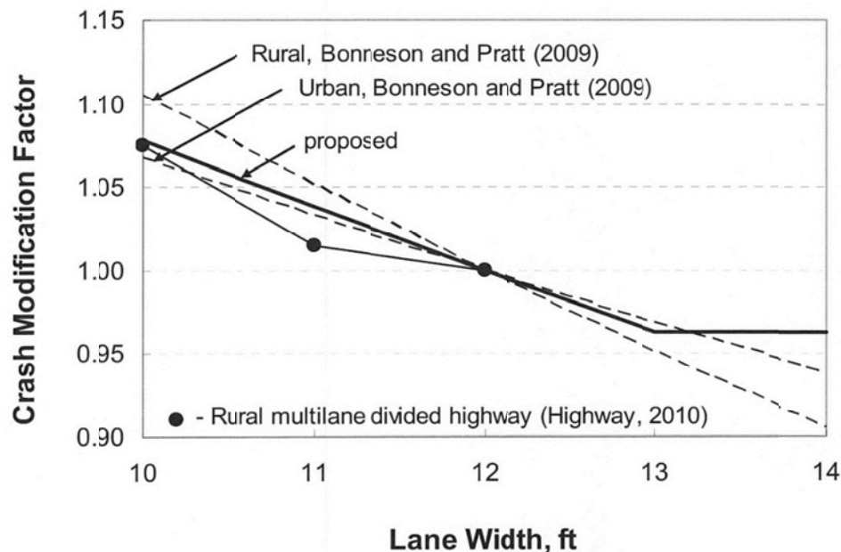
Figure 40. Crash Modification Factor for Lane Widths on Freeways. Source: HSM
