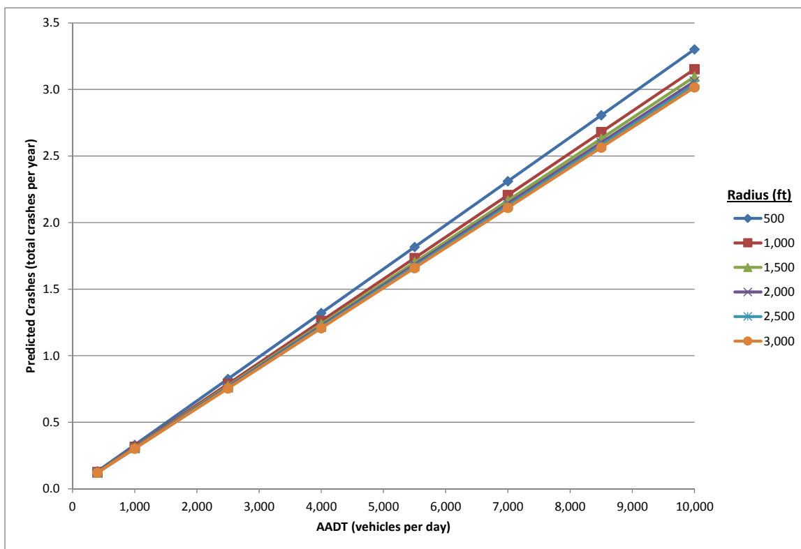
Figure C-4. Annual Predicted Crash Frequency by Radius for a 45° Deflection Angle
