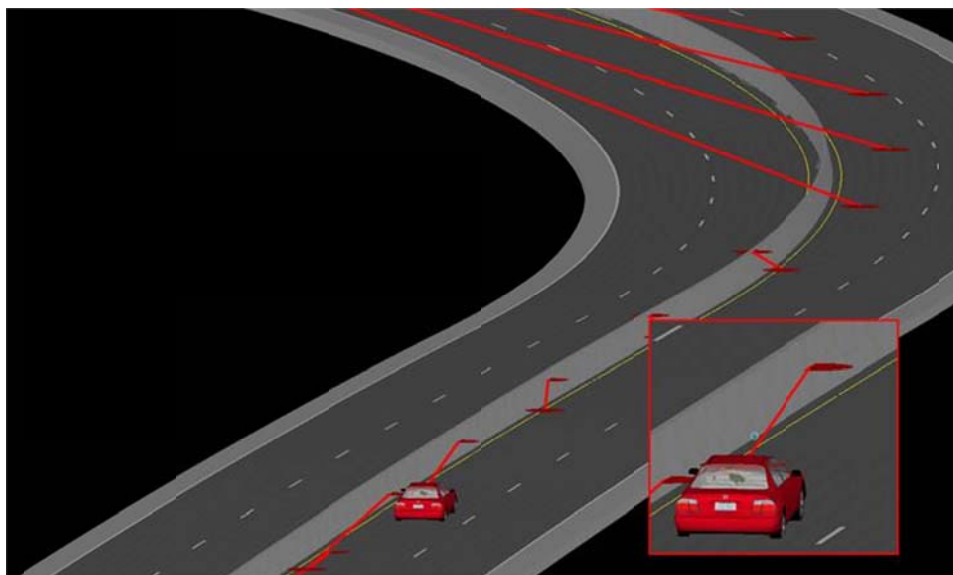
Figure 39. BIM Output to Evaluate Sight Lines along Curved Roadway with Barrier
