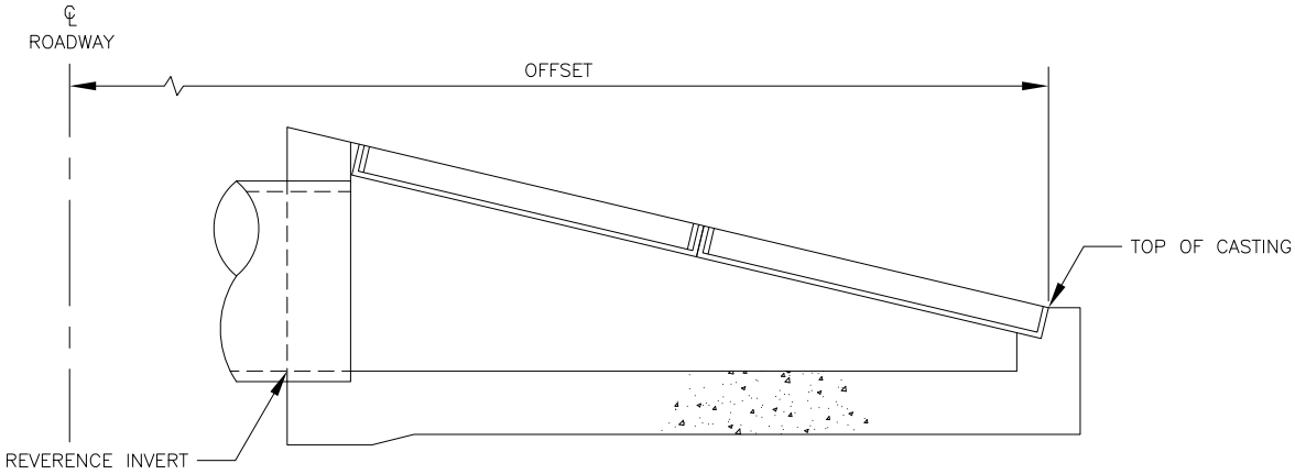
TYPICAL TYPE "C" INLET BOX SECTION
