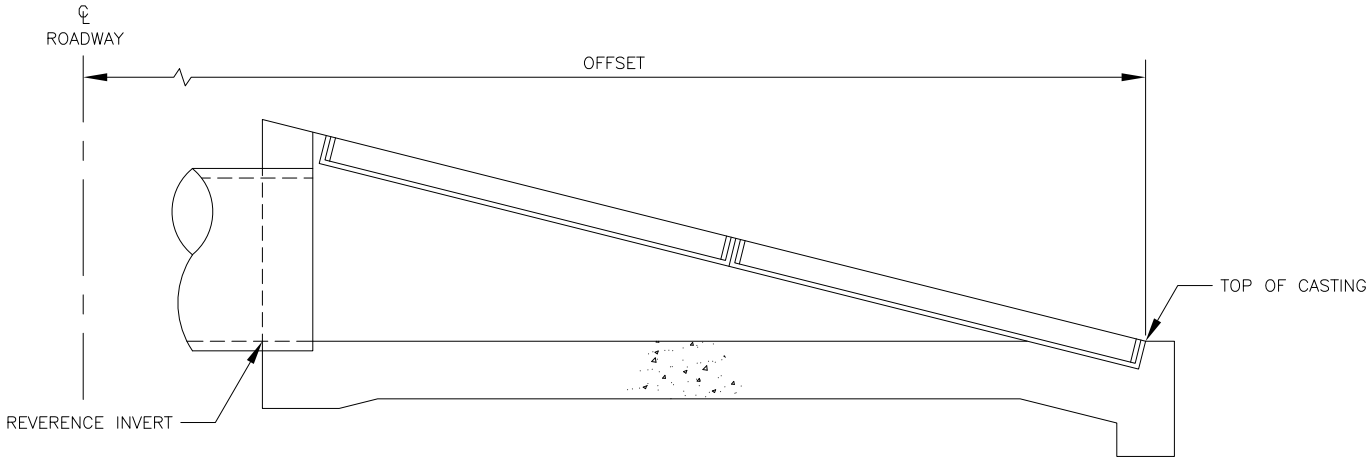
TYPICAL TYPE "D" INLET BOX SECTION
