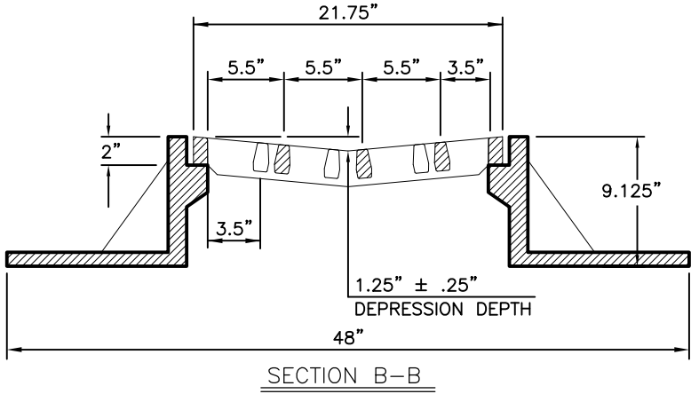
HIGH CAPACITY INLET DETAIL
