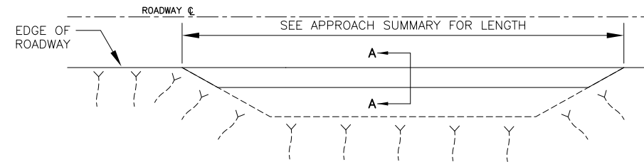
PULLOUT PLAN VIEW
