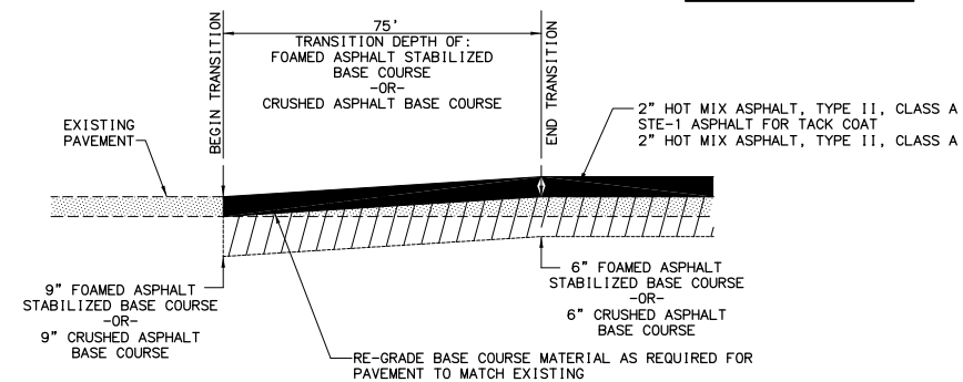
ROADWAY PAVEMENT TRANSITION TO EXISTING PAVEMENT
