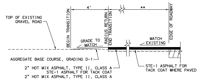
GRAVEL APPROACH TRANSITION
