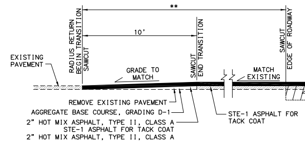
PAVED APPROACH TRANSITION
