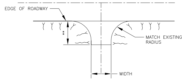
APPROACH PLAN VIEW
