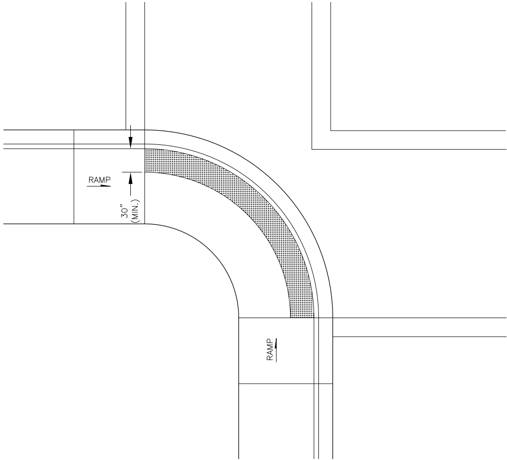
BLEND E D CURB RAMP
