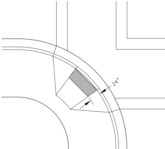
SHARED CURB RAMP
