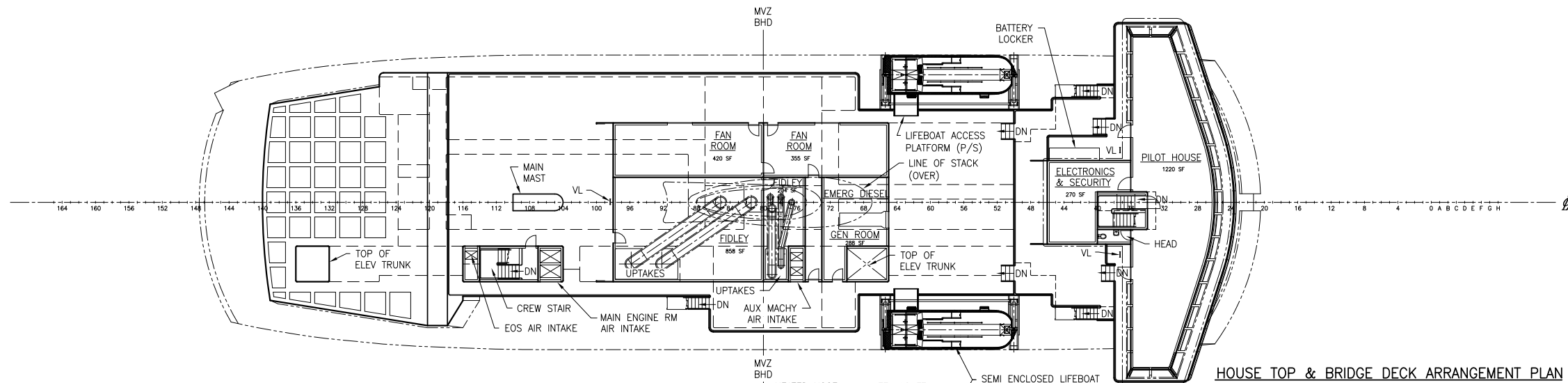
HOUSE TOP & BRIDGE DECK ARRANGEMENT PLAN
