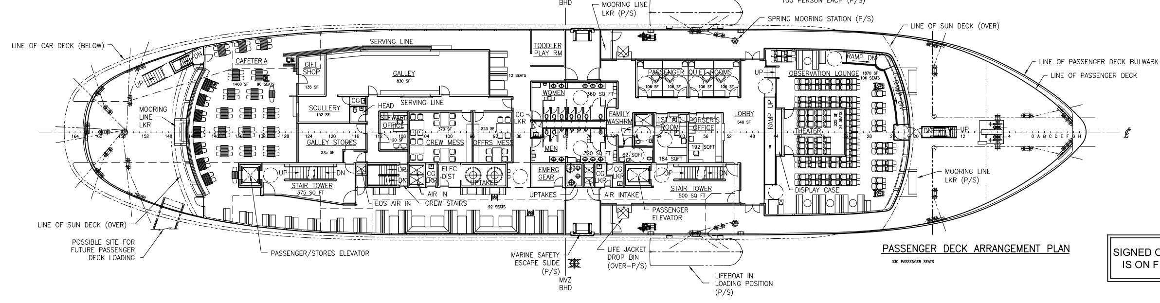
SUN DECK ARRANGEMENT PLAN
