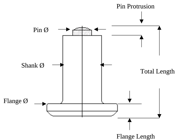
Figure 2.1. Stud Construction, Single Flange (Simon Company Group 2003)
