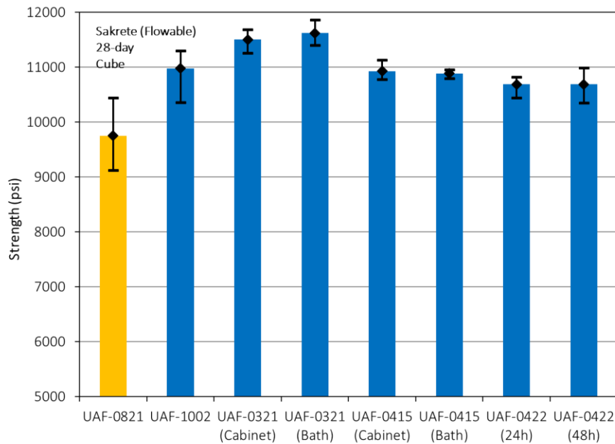
Figure 3-1. Compressive strength of Sakrete® cubes in Round 3 and Round 4
