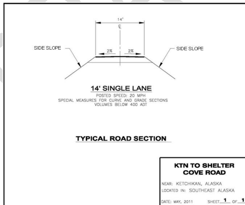
Figure #4. Typical Road Section
