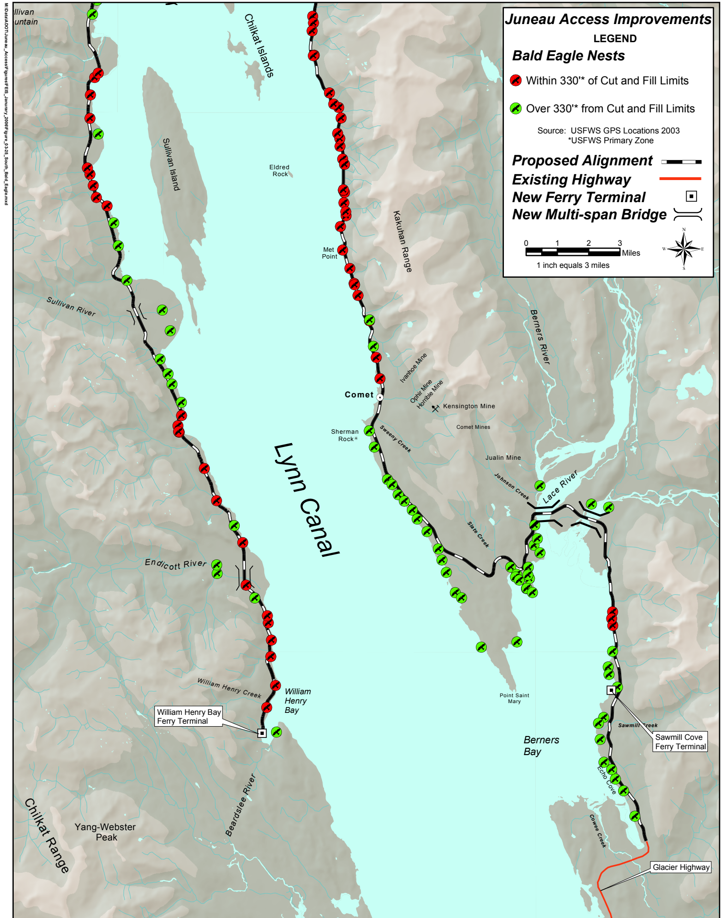
Figure 3-25 Bald Eagle Nest Locations at Southern End of Lynn Canal
