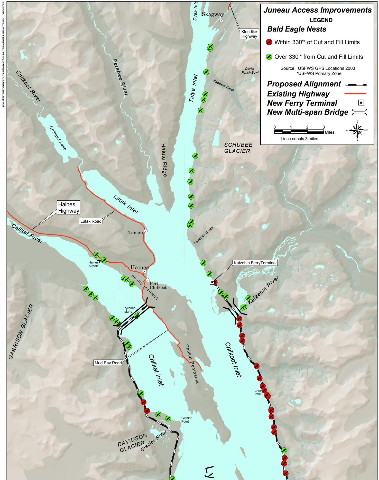
Figure 3-24 Bald Eagle Nest Locations at Northern End of Lynn Canal
