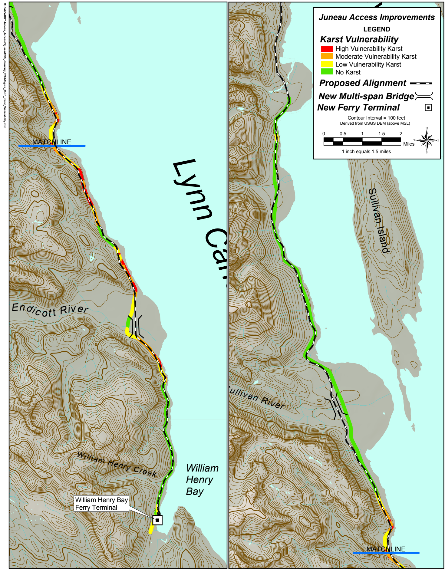
Figure 3-11 Karst Vulnerability for West Lynn Canal Area
