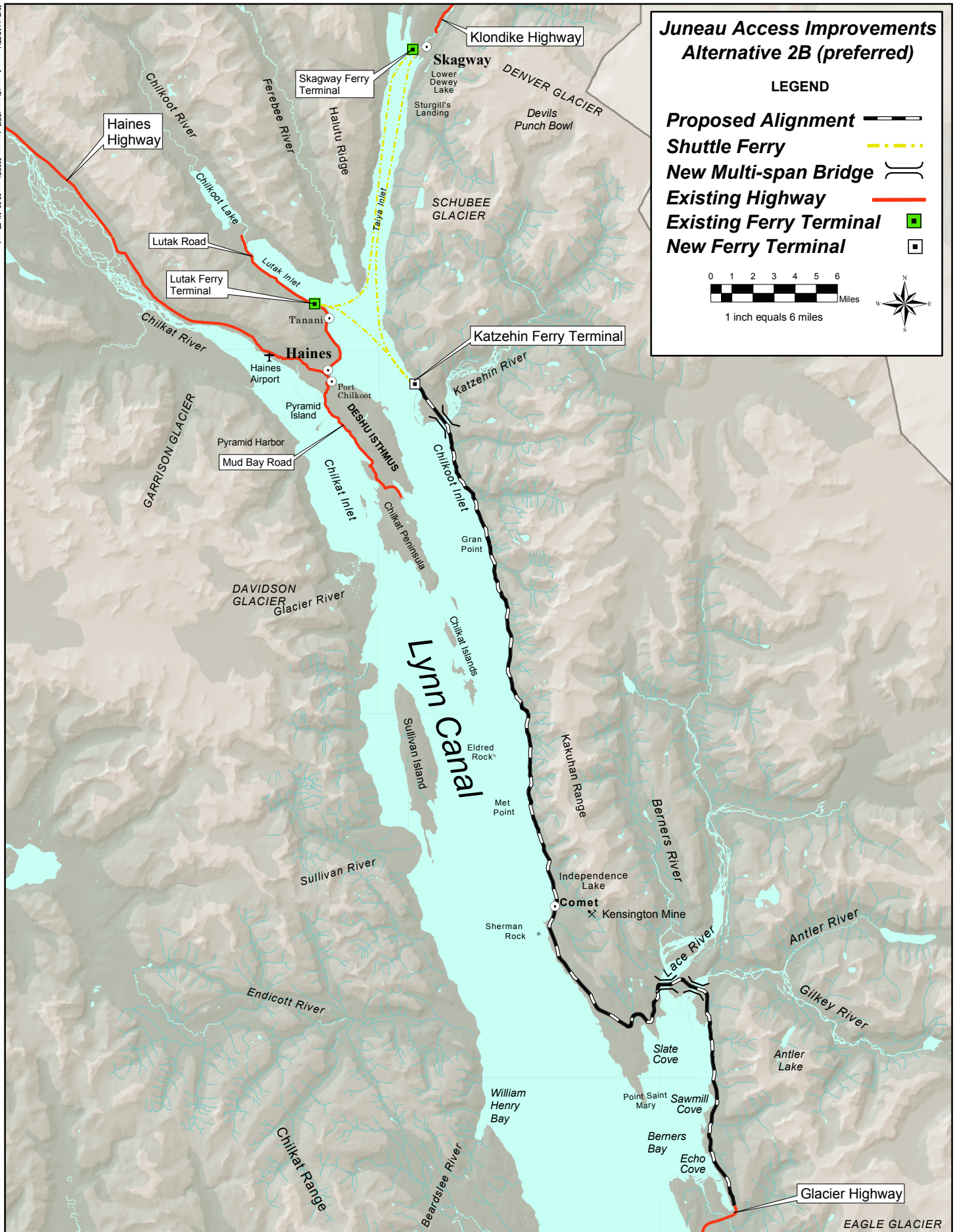
Figure 2-6 Alternative 2B (preferred): East Lynn Canal Highway to Katzehin Ferry Terminal with Shuttles to Haines & Skagway
