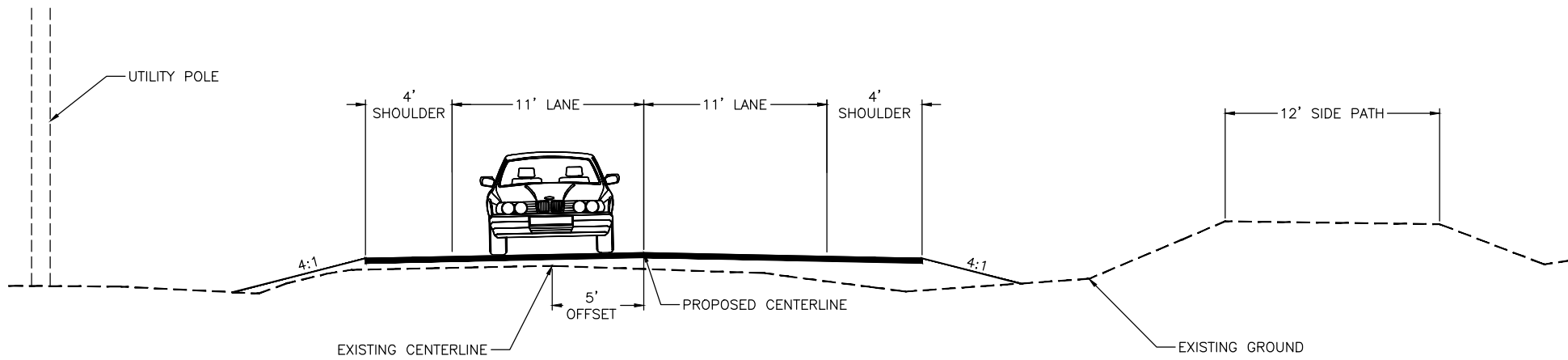
MILLER HILL ROAD 11' LANE W/ 4' SHOULDER PROPOSED CROSS SECTION
