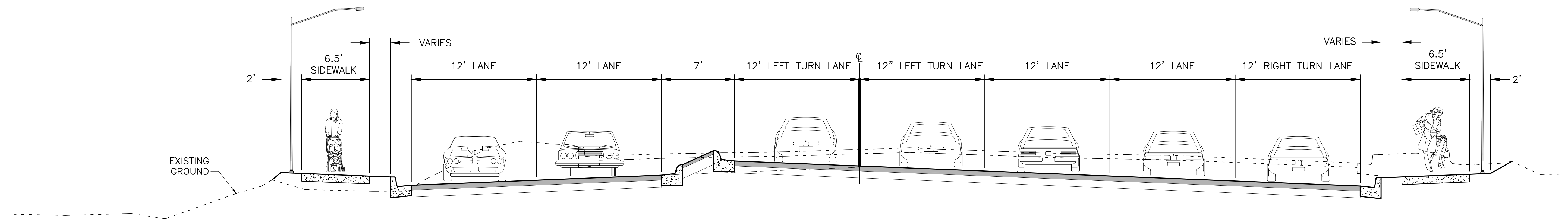
GEIST ROAD TYPICAL
