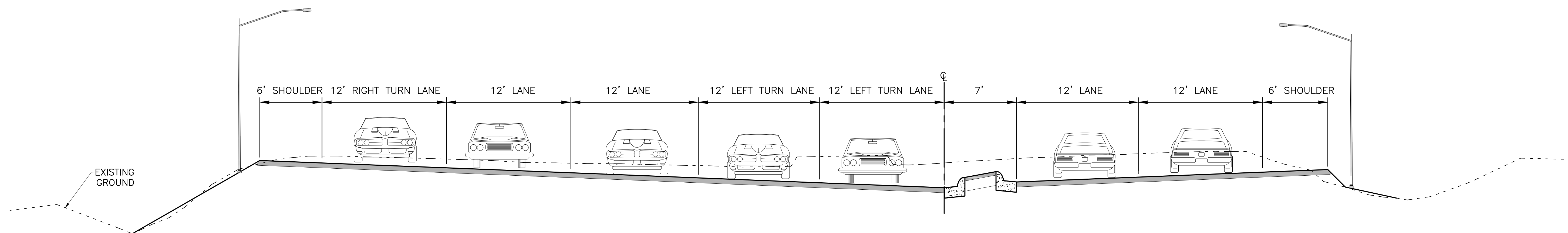
JOHANSEN EXPRESSWAY TYPICAL
