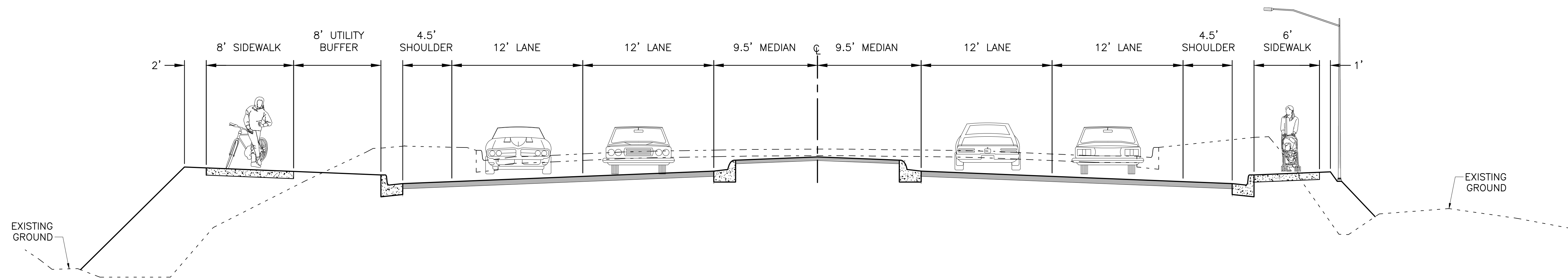
UNIVERSITY AVENUE TYPICAL
