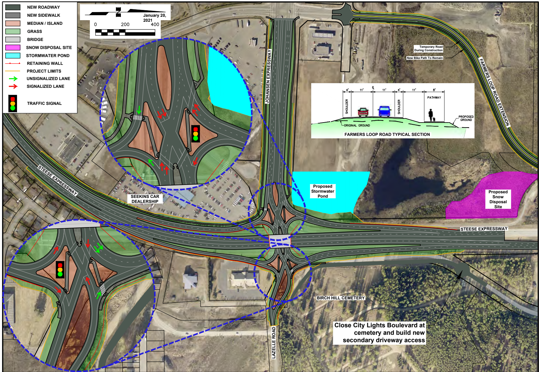
Diverging Diamond Alternative
