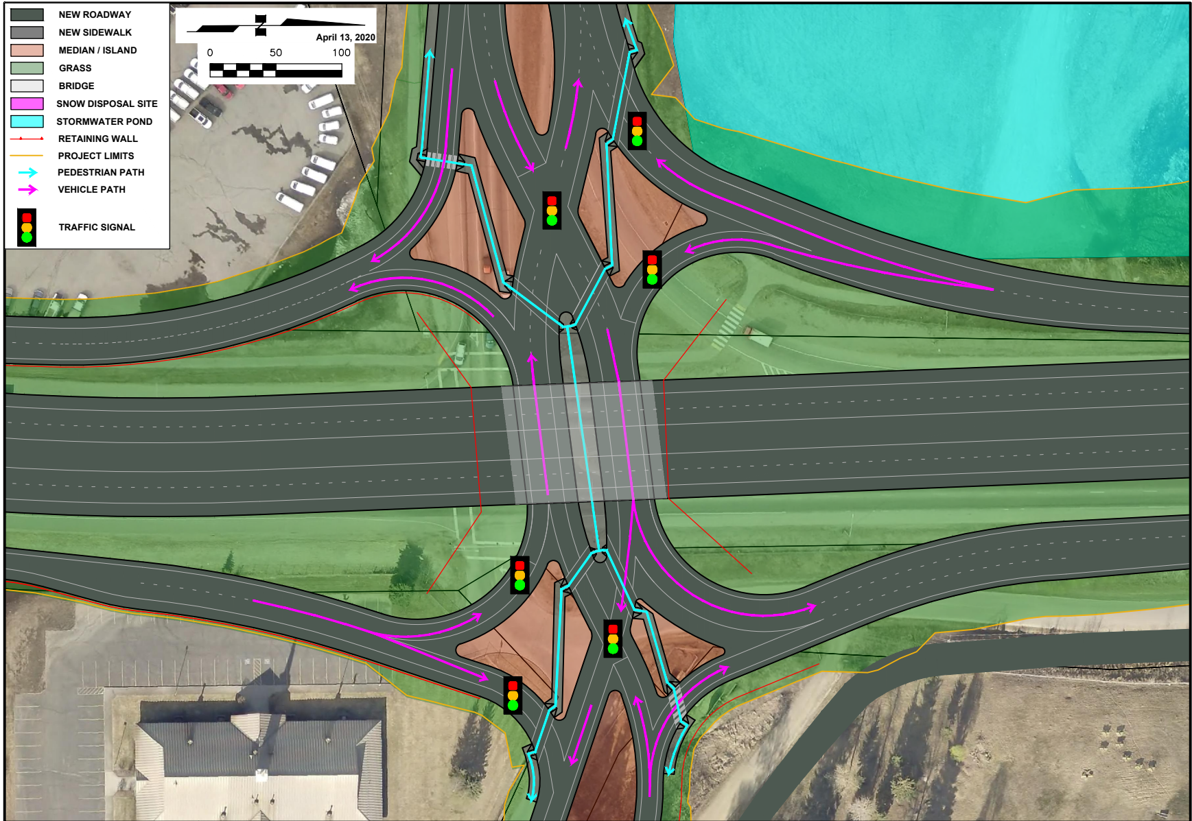
Diverging Diamond Intersection Operations
