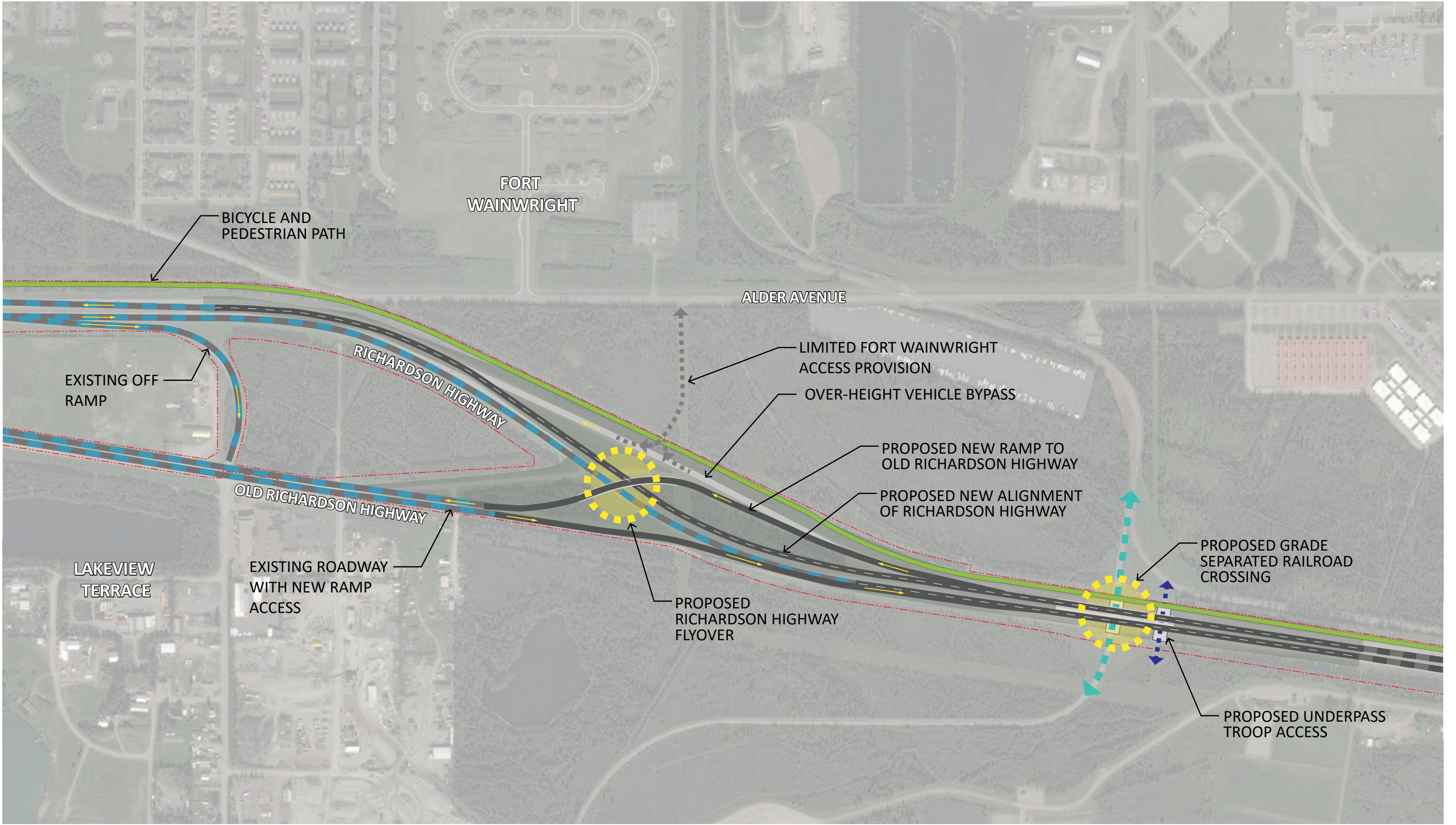
Flyover Concept
