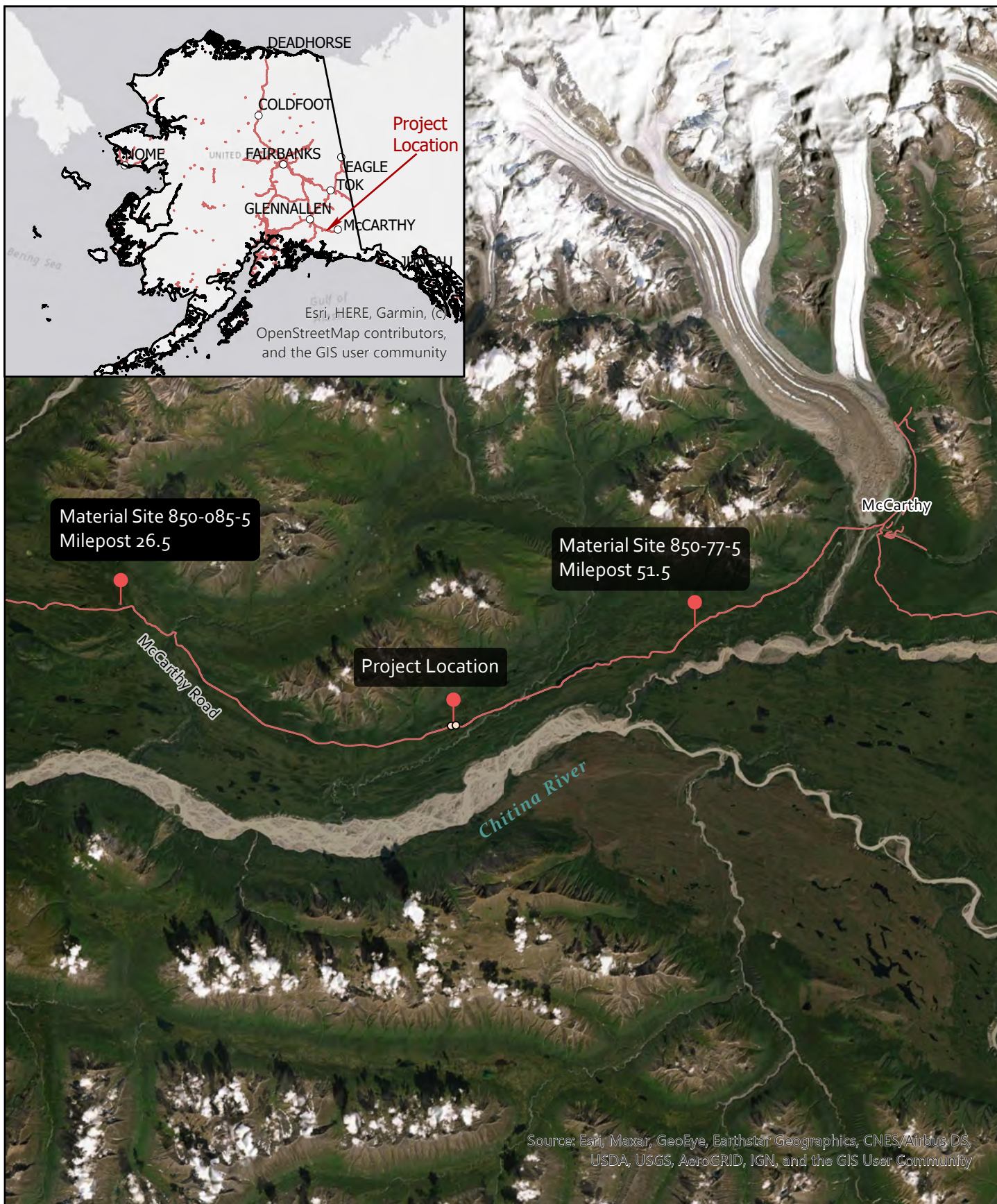
McCarthy Road MP 41 Crystal Creek Culvert Replacement Location Map McCarthy Road, Alaska Figure 1
