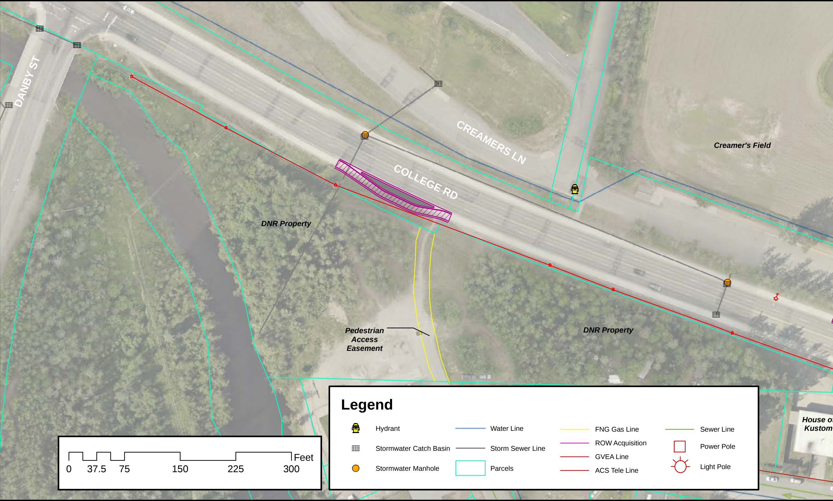
KATHRYN AVENUE SOUTH/FIGURE 4
