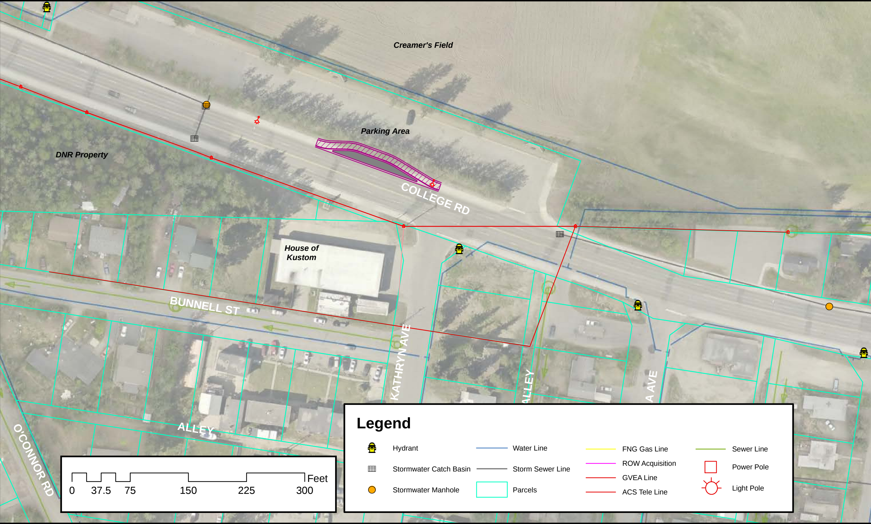
KATHRYN AVENUE NORTH/FIGURE 5
